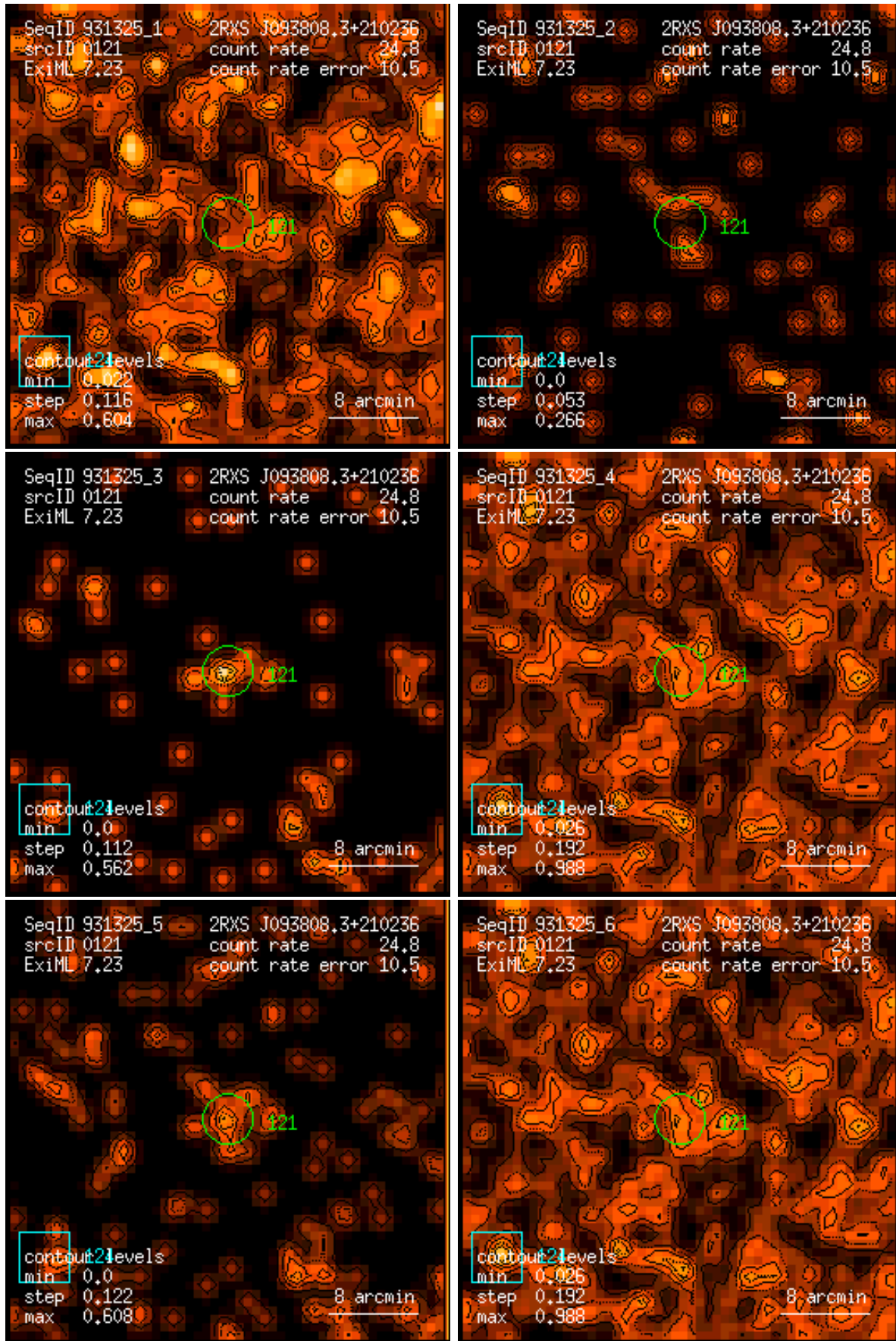
Figure 121: RASS 931325: detection 0121: band rate images, Gaussian filter: (1) PSPC channels 11 – 41, (2) 52 – 90, (3) 91 – 201, (4) 11 – 235, (5) 52 – 201, (6) 11 – 201. Broad band rates in counts/ks. Band rate contour levels in counts/ks/arcmin 2 .
