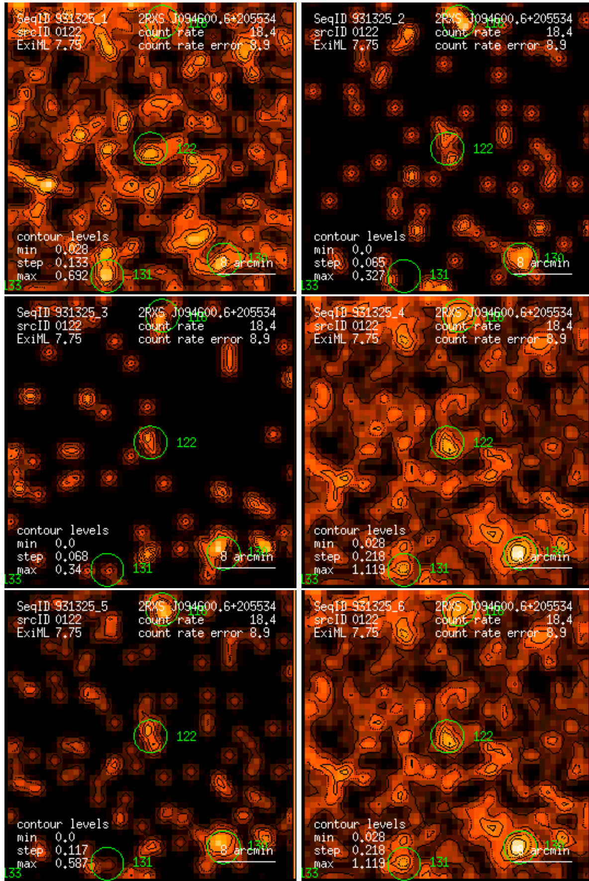
Figure 122: RASS 931325: detection 0122: band rate images, Gaussian filter: (1) PSPC channels 11 – 41, (2) 52 – 90, (3) 91 – 201, (4) 11 – 235, (5) 52 – 201, (6) 11 – 201. Broad band rates in counts/ks. Band rate contour levels in counts/ks/arcmin 2 .
