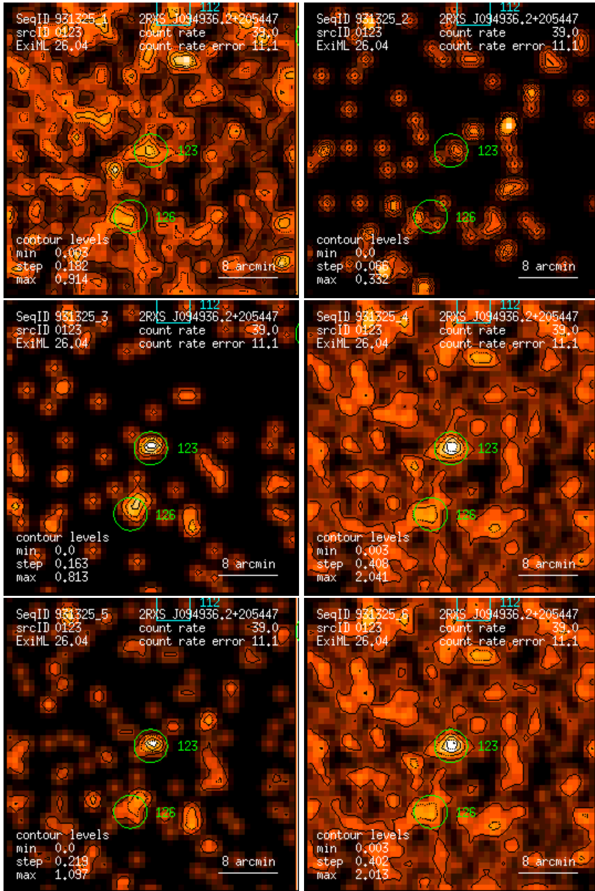
Figure 123: RASS 931325: detection 0123: band rate images, Gaussian filter: (1) PSPC channels 11 – 41, (2) 52 – 90, (3) 91 – 201, (4) 11 – 235, (5) 52 – 201, (6) 11 – 201. Broad band rates in counts/ks. Band rate contour levels in counts/ks/arcmin 2 .
