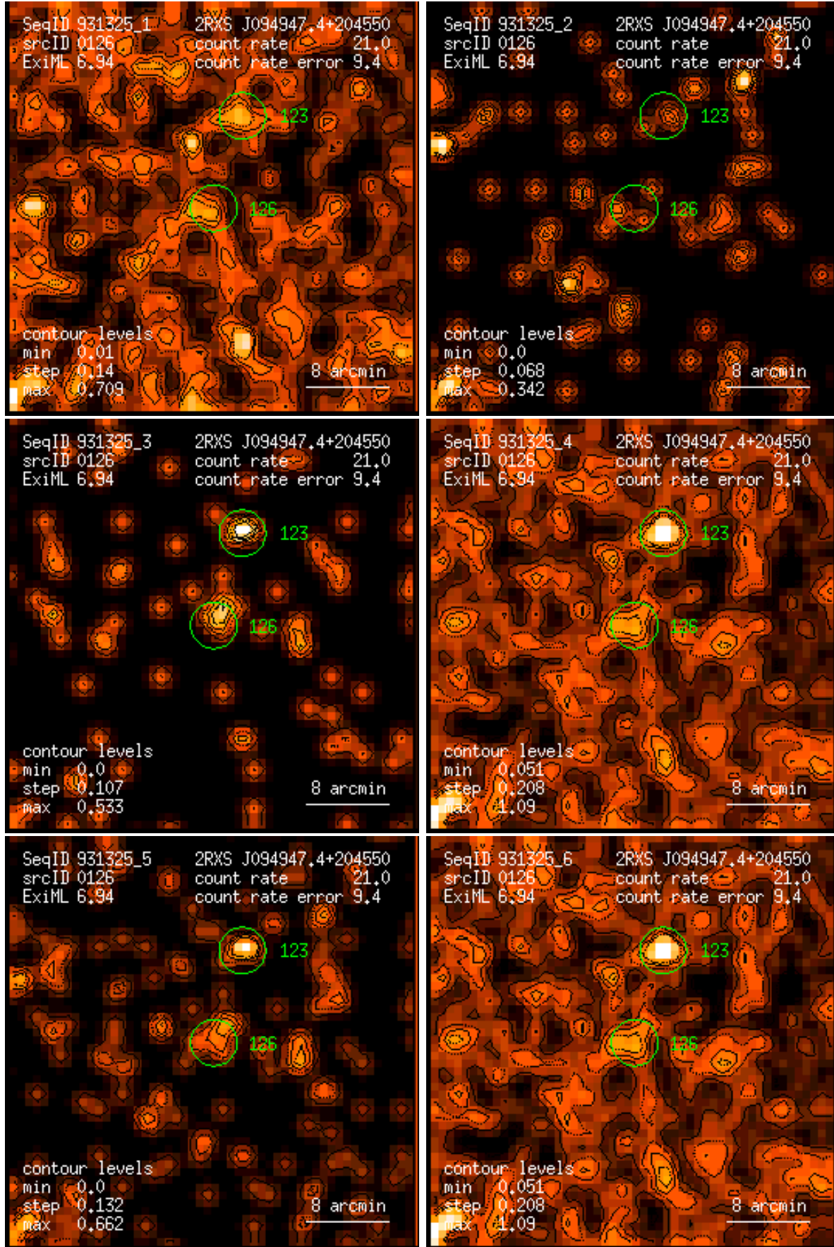
Figure 126: RASS 931325: detection 0126: band rate images, Gaussian filter: (1) PSPC channels 11 – 41, (2) 52 – 90, (3) 91 – 201, (4) 11 – 235, (5) 52 – 201, (6) 11 – 201. Broad band rates in counts/ks. Band rate contour levels in counts/ks/arcmin 2 .
