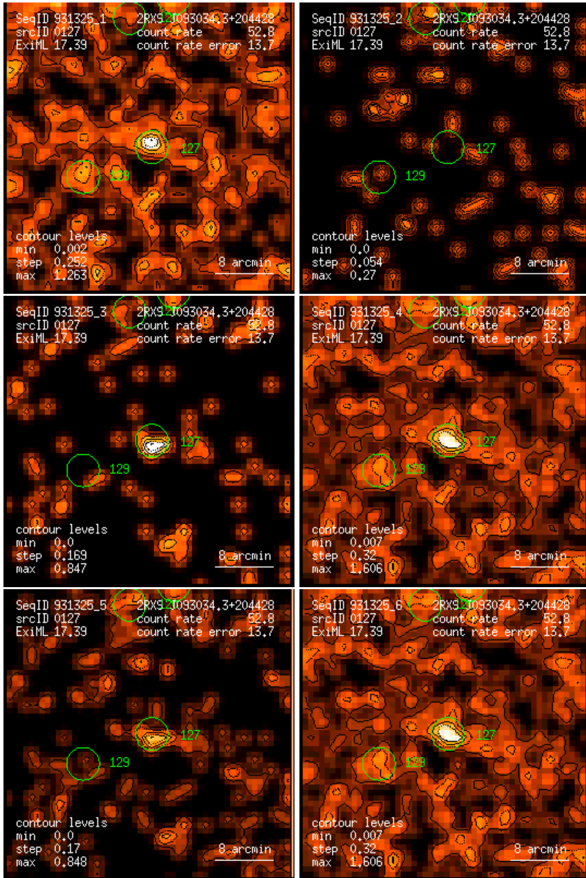
Figure 127: RASS 931325: detection 0127: band rate images, Gaussian filter: (1) PSPC channels 11 – 41, (2) 52 – 90, (3) 91 – 201, (4) 11 – 235, (5) 52 – 201, (6) 11 – 201. Broad band rates in counts/ks. Band rate contour levels in counts/ks/arcmin 2 .
