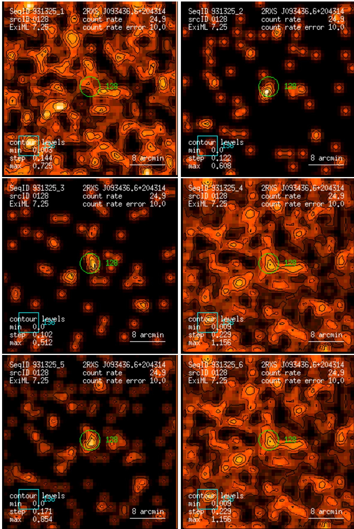
Figure 128: RASS 931325: detection 0128: band rate images, Gaussian filter: (1) PSPC channels 11 – 41, (2) 52 – 90, (3) 91 – 201, (4) 11 – 235, (5) 52 – 201, (6) 11 – 201. Broad band rates in counts/ks. Band rate contour levels in counts/ks/arcmin 2 .
