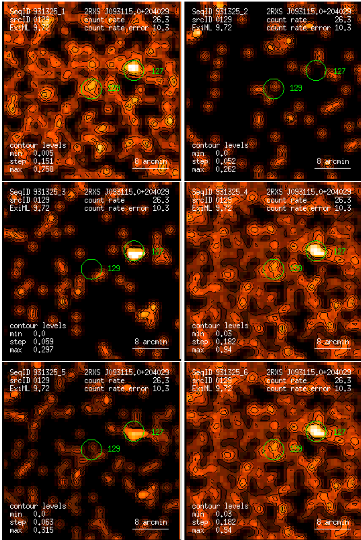
Figure 129: RASS 931325: detection 0129: band rate images, Gaussian filter: (1) PSPC channels 11 – 41, (2) 52 – 90, (3) 91 – 201, (4) 11 – 235, (5) 52 – 201, (6) 11 – 201. Broad band rates in counts/ks. Band rate contour levels in counts/ks/arcmin 2 .
