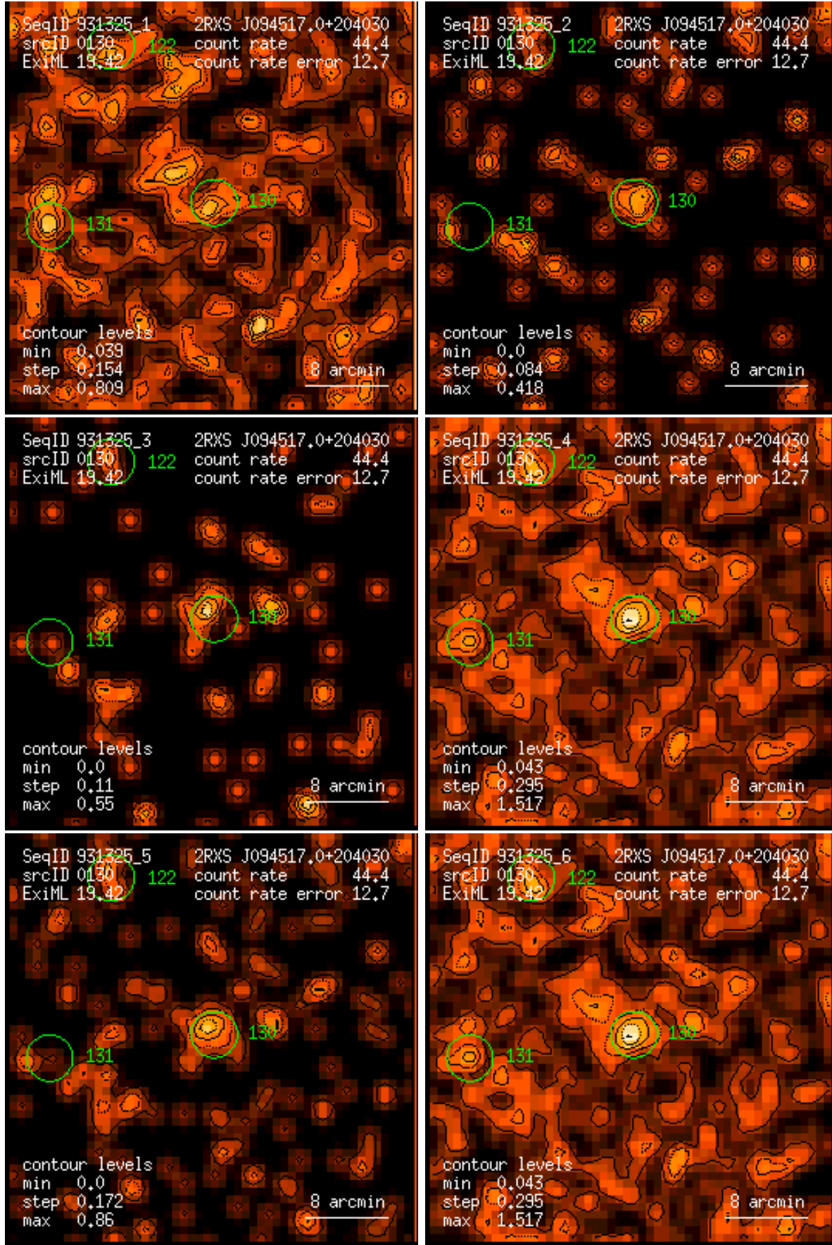
Figure 130: RASS 931325: detection 0130: band rate images, Gaussian filter: (1) PSPC channels 11 – 41, (2) 52 – 90, (3) 91 – 201, (4) 11 – 235, (5) 52 – 201, (6) 11 – 201. Broad band rates in counts/ks. Band rate contour levels in counts/ks/arcmin 2 .
