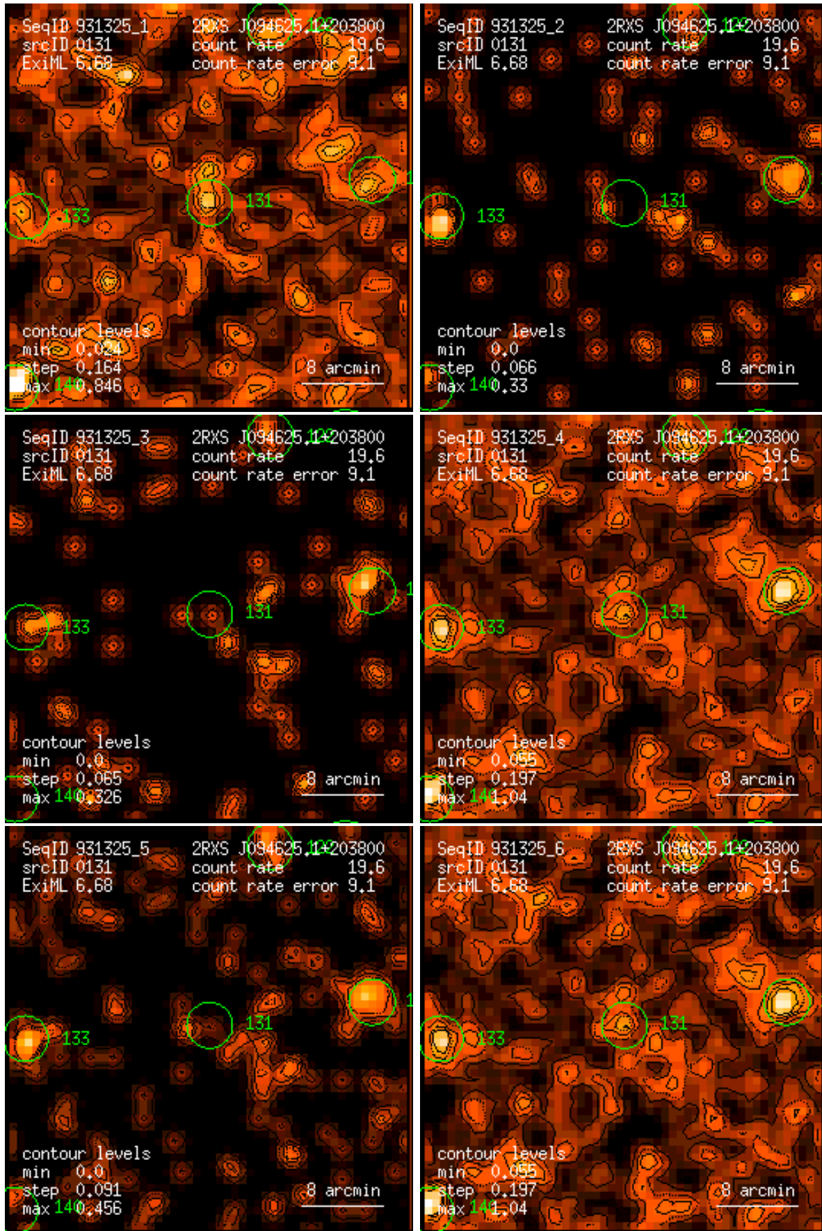
Figure 131: RASS 931325: detection 0131: band rate images, Gaussian filter: (1) PSPC channels 11 – 41, (2) 52 – 90, (3) 91 – 201, (4) 11 – 235, (5) 52 – 201, (6) 11 – 201. Broad band rates in counts/ks. Band rate contour levels in counts/ks/arcmin 2 .
