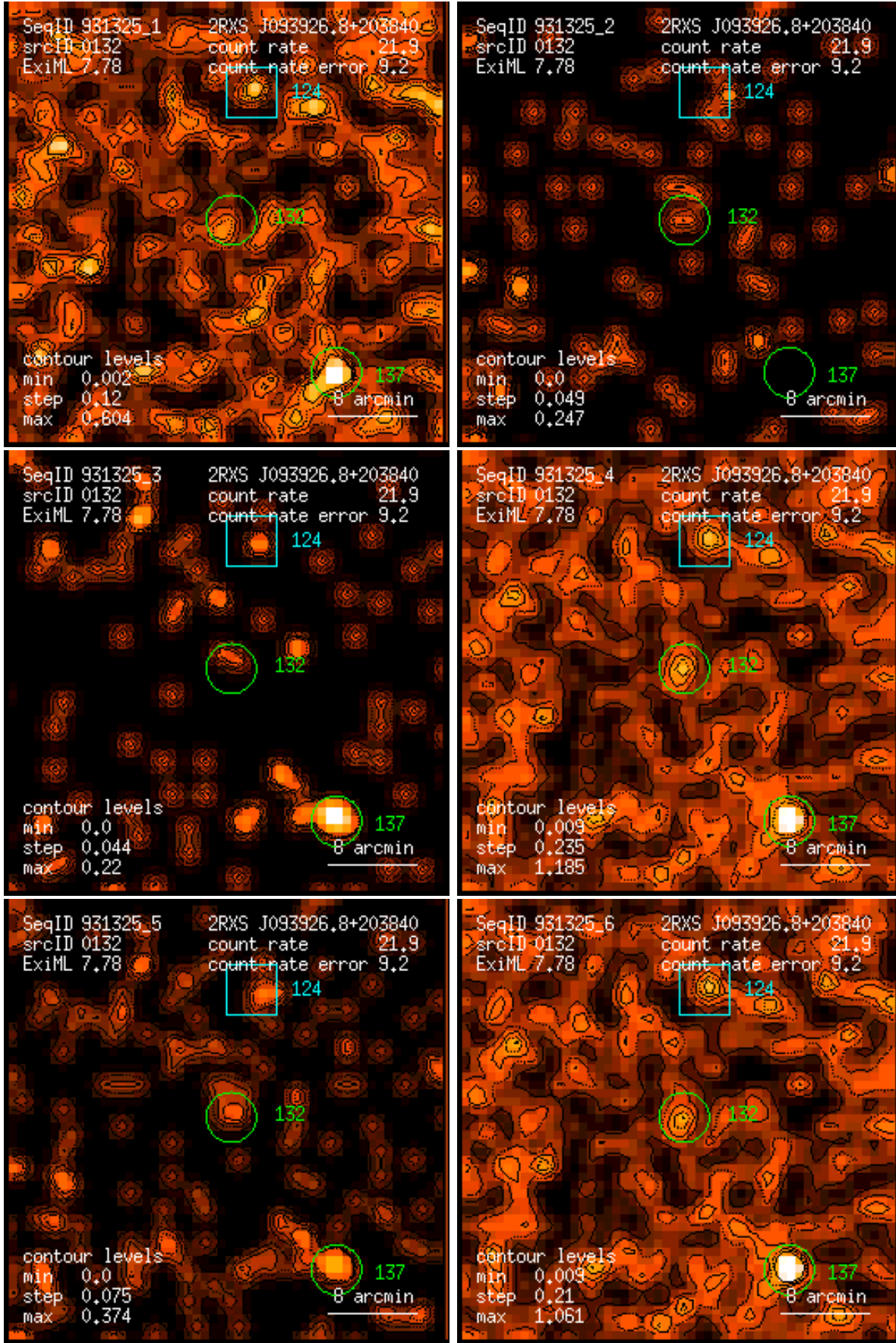
Figure 132: RASS 931325: detection 0132: band rate images, Gaussian filter: (1) PSPC channels 11 – 41, (2) 52 – 90, (3) 91 – 201, (4) 11 – 235, (5) 52 – 201, (6) 11 – 201. Broad band rates in counts/ks. Band rate contour levels in counts/ks/arcmin 2 .
