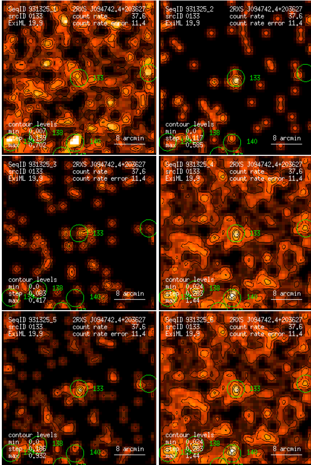
Figure 133: RASS 931325: detection 0133: band rate images, Gaussian filter: (1) PSPC channels 11 – 41, (2) 52 – 90, (3) 91 – 201, (4) 11 – 235, (5) 52 – 201, (6) 11 – 201. Broad band rates in counts/ks. Band rate contour levels in counts/ks/arcmin 2 .
