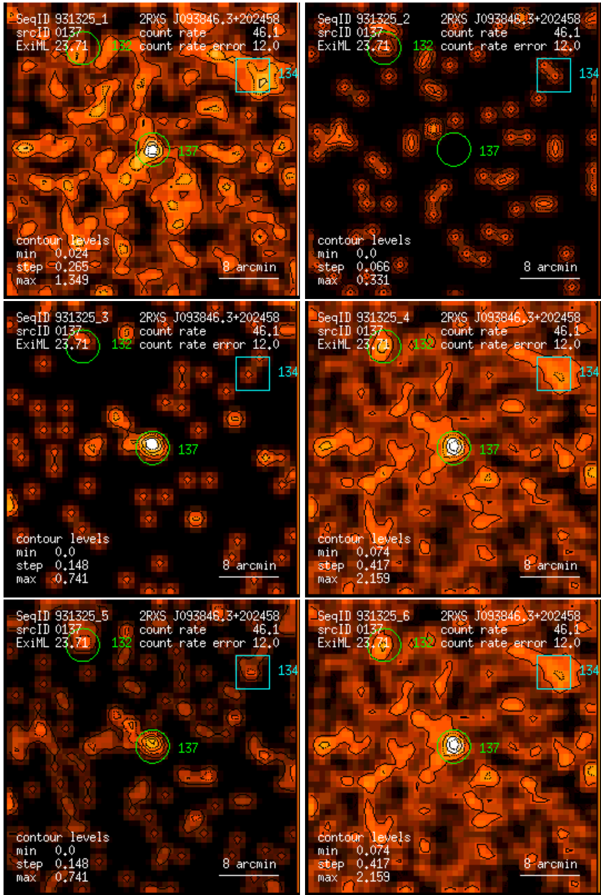
Figure 137: RASS 931325: detection 0137: band rate images, Gaussian filter: (1) PSPC channels 11 – 41, (2) 52 – 90, (3) 91 – 201, (4) 11 – 235, (5) 52 – 201, (6) 11 – 201. Broad band rates in counts/ks. Band rate contour levels in counts/ks/arcmin 2 .
