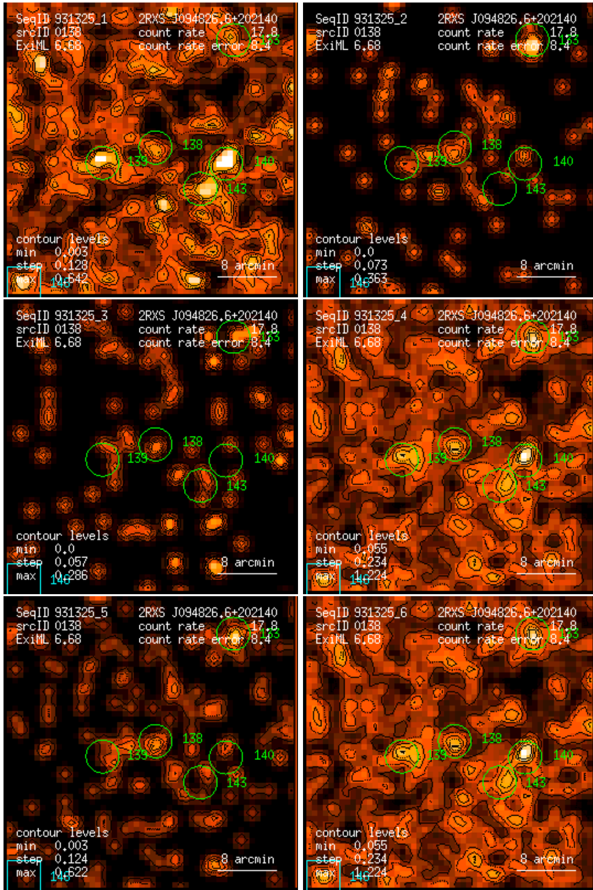
Figure 138: RASS 931325: detection 0138: band rate images, Gaussian filter: (1) PSPC channels 11 – 41, (2) 52 – 90, (3) 91 – 201, (4) 11 – 235, (5) 52 – 201, (6) 11 – 201. Broad band rates in counts/ks. Band rate contour levels in counts/ks/arcmin 2 .
