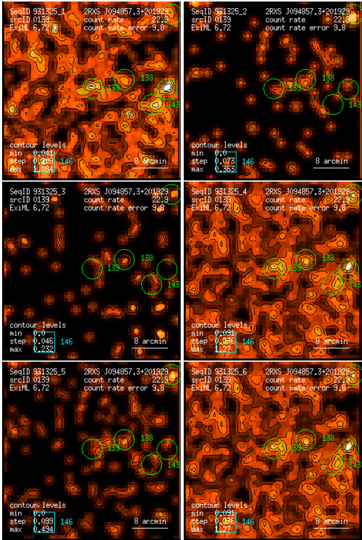
Figure 139: RASS 931325: detection 0139: band rate images, Gaussian filter: (1) PSPC channels 11 – 41, (2) 52 – 90, (3) 91 – 201, (4) 11 – 235, (5) 52 – 201, (6) 11 – 201. Broad band rates in counts/ks. Band rate contour levels in counts/ks/arcmin 2 .
