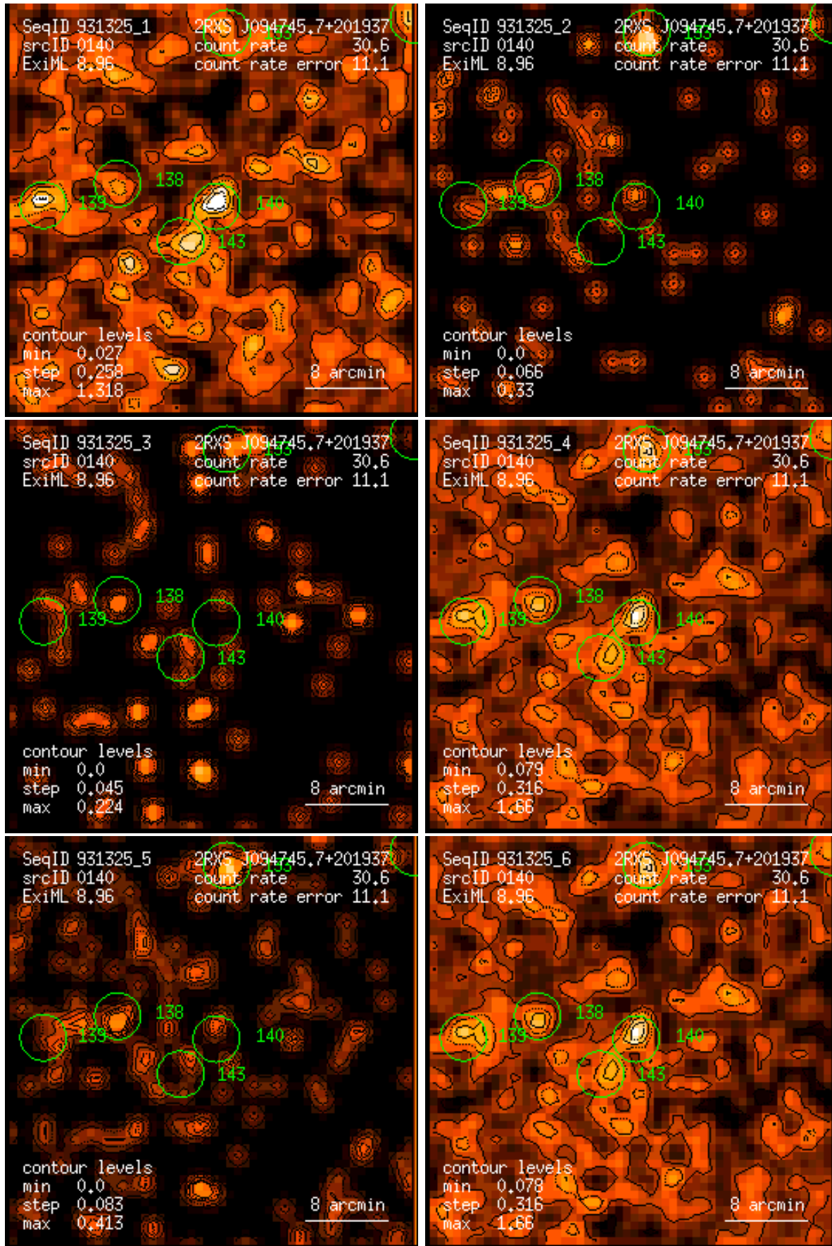
Figure 140: RASS 931325: detection 0140: band rate images, Gaussian filter: (1) PSPC channels 11 – 41, (2) 52 – 90, (3) 91 – 201, (4) 11 – 235, (5) 52 – 201, (6) 11 – 201. Broad band rates in counts/ks. Band rate contour levels in counts/ks/arcmin 2 .
