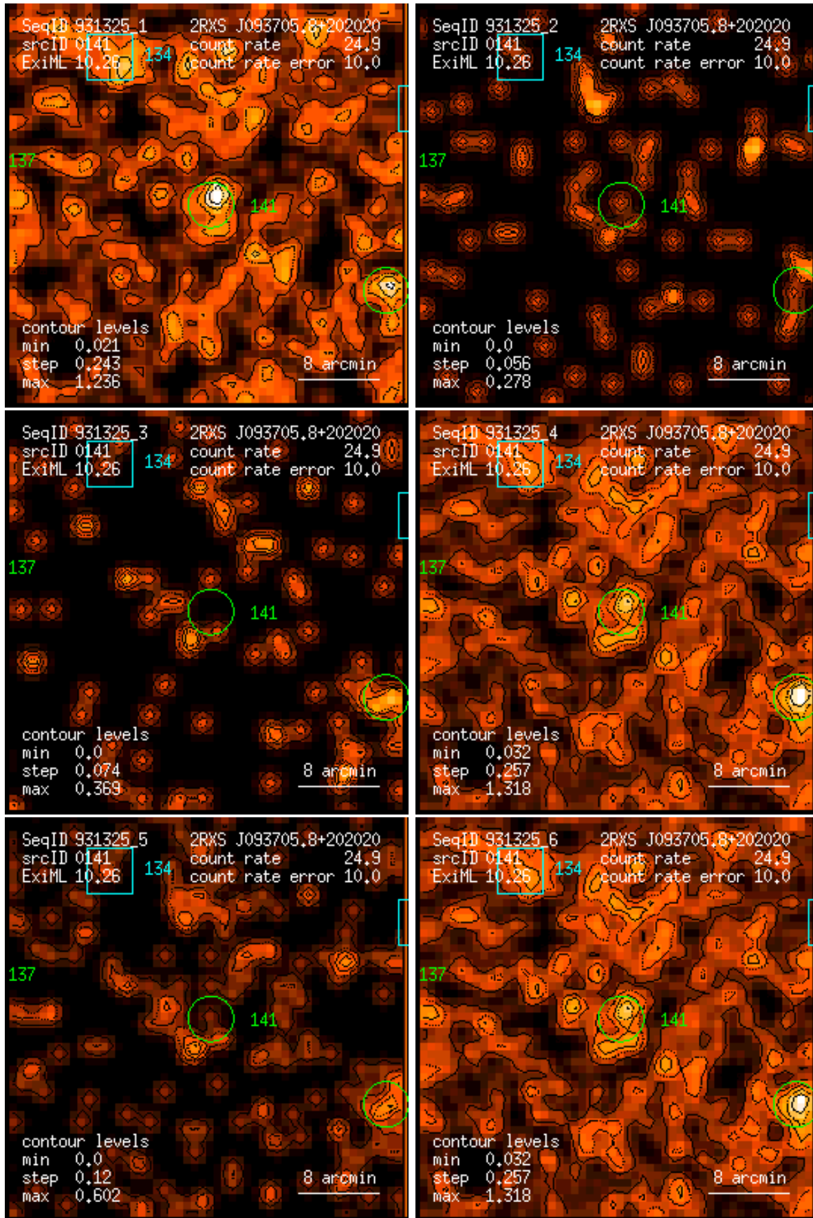
Figure 141: RASS 931325: detection 0141: band rate images, Gaussian filter: (1) PSPC channels 11 – 41, (2) 52 – 90, (3) 91 – 201, (4) 11 – 235, (5) 52 – 201, (6) 11 – 201. Broad band rates in counts/ks. Band rate contour levels in counts/ks/arcmin 2 .
