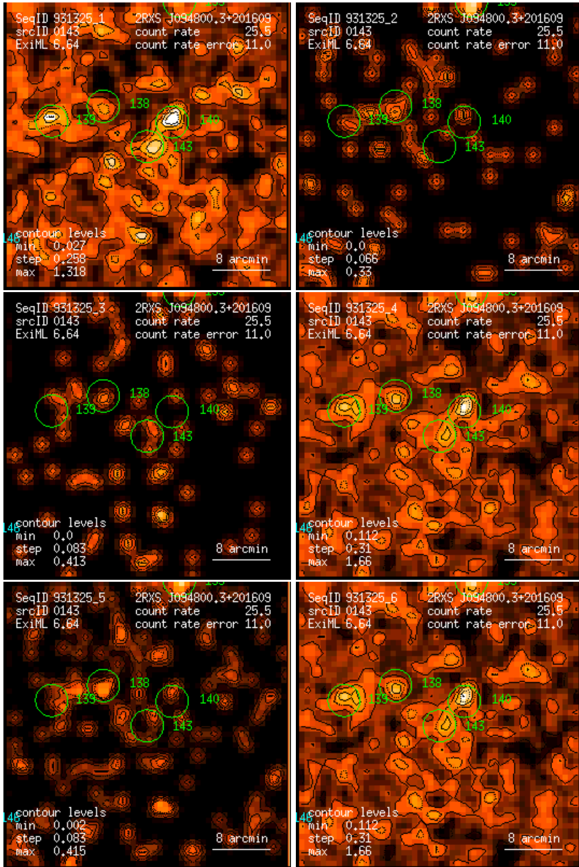
Figure 143: RASS 931325: detection 0143: band rate images, Gaussian filter: (1) PSPC channels 11 – 41, (2) 52 – 90, (3) 91 – 201, (4) 11 – 235, (5) 52 – 201, (6) 11 – 201. Broad band rates in counts/ks. Band rate contour levels in counts/ks/arcmin 2 .
