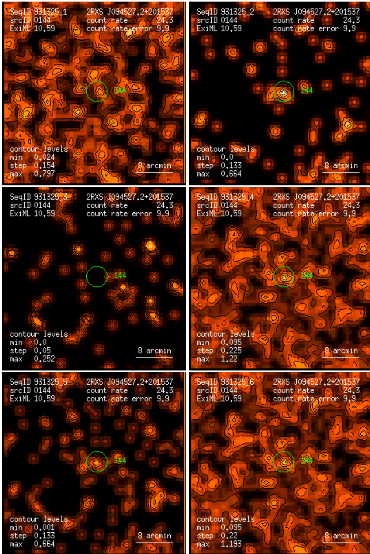
Figure 144: RASS 931325: detection 0144: band rate images, Gaussian filter: (1) PSPC channels 11 – 41, (2) 52 – 90, (3) 91 – 201, (4) 11 – 235, (5) 52 – 201, (6) 11 – 201. Broad band rates in counts/ks. Band rate contour levels in counts/ks/arcmin 2 .
