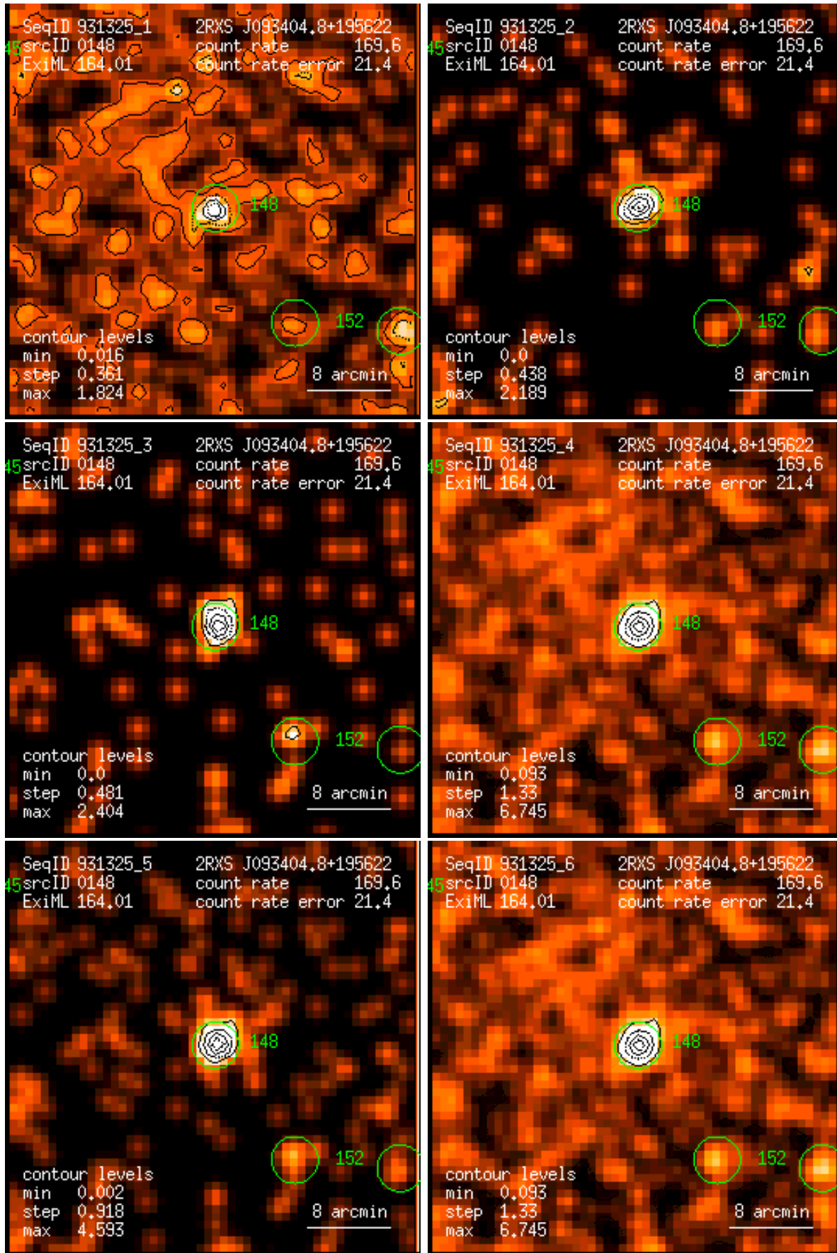
Figure 148: RASS 931325: detection 0148: band rate images, Gaussian filter: (1) PSPC channels 11 – 41, (2) 52 – 90, (3) 91 – 201, (4) 11 – 235, (5) 52 – 201, (6) 11 – 201. Broad band rates in counts/ks. Band rate contour levels in counts/ks/arcmin 2 .
