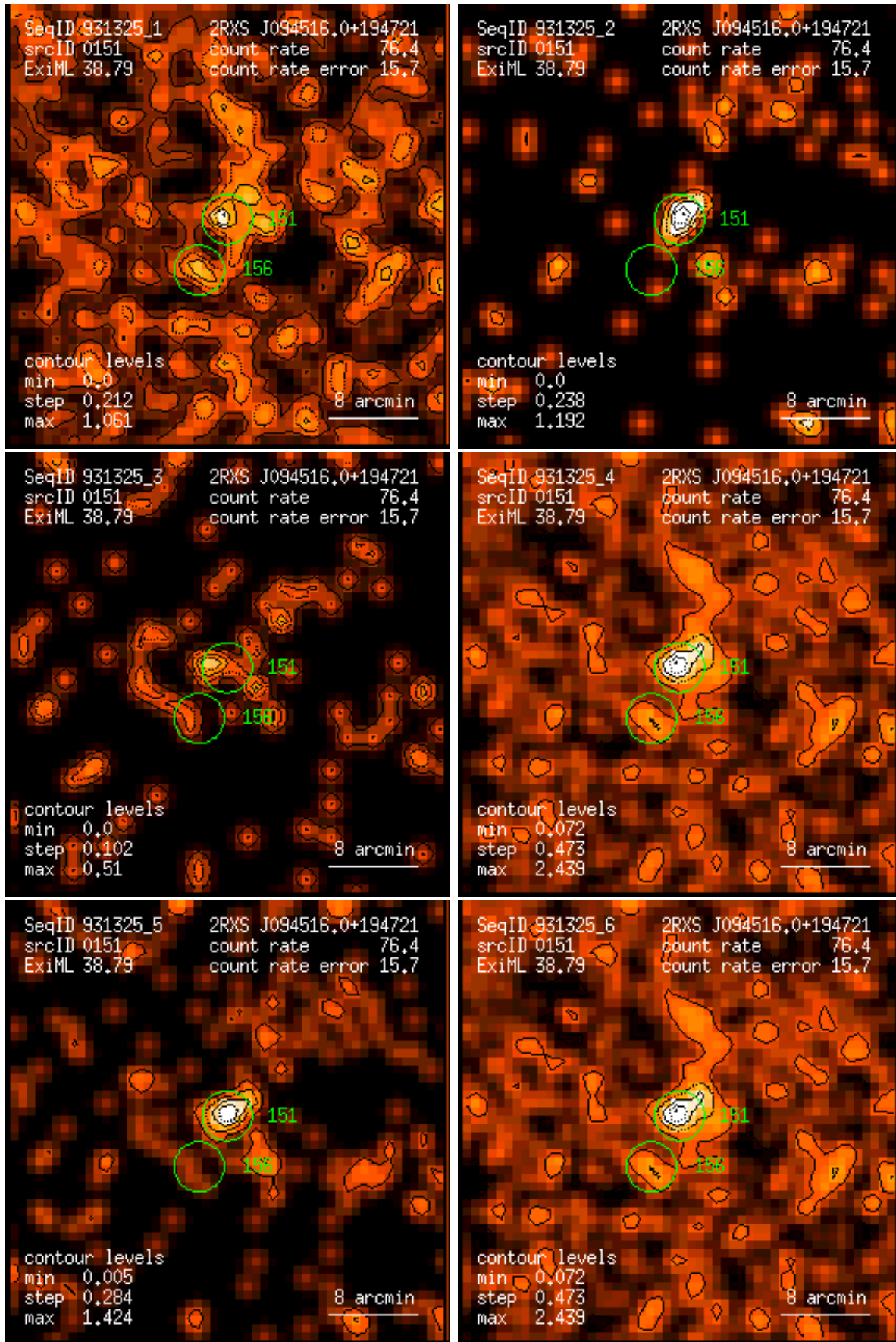
Figure 151: RASS 931325: detection 0151: band rate images, Gaussian filter: (1) PSPC channels 11 – 41, (2) 52 – 90, (3) 91 – 201, (4) 11 – 235, (5) 52 – 201, (6) 11 – 201. Broad band rates in counts/ks. Band rate contour levels in counts/ks/arcmin 2 .
