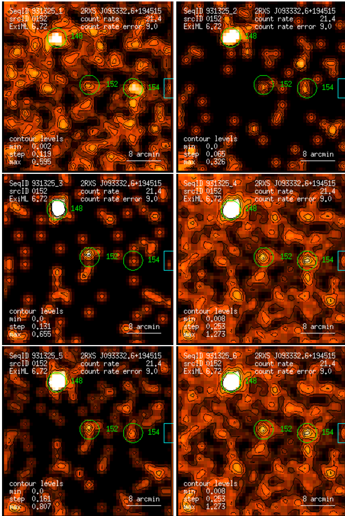
Figure 152: RASS 931325: detection 0152: band rate images, Gaussian filter: (1) PSPC channels 11 – 41, (2) 52 – 90, (3) 91 – 201, (4) 11 – 235, (5) 52 – 201, (6) 11 – 201. Broad band rates in counts/ks. Band rate contour levels in counts/ks/arcmin 2 .
