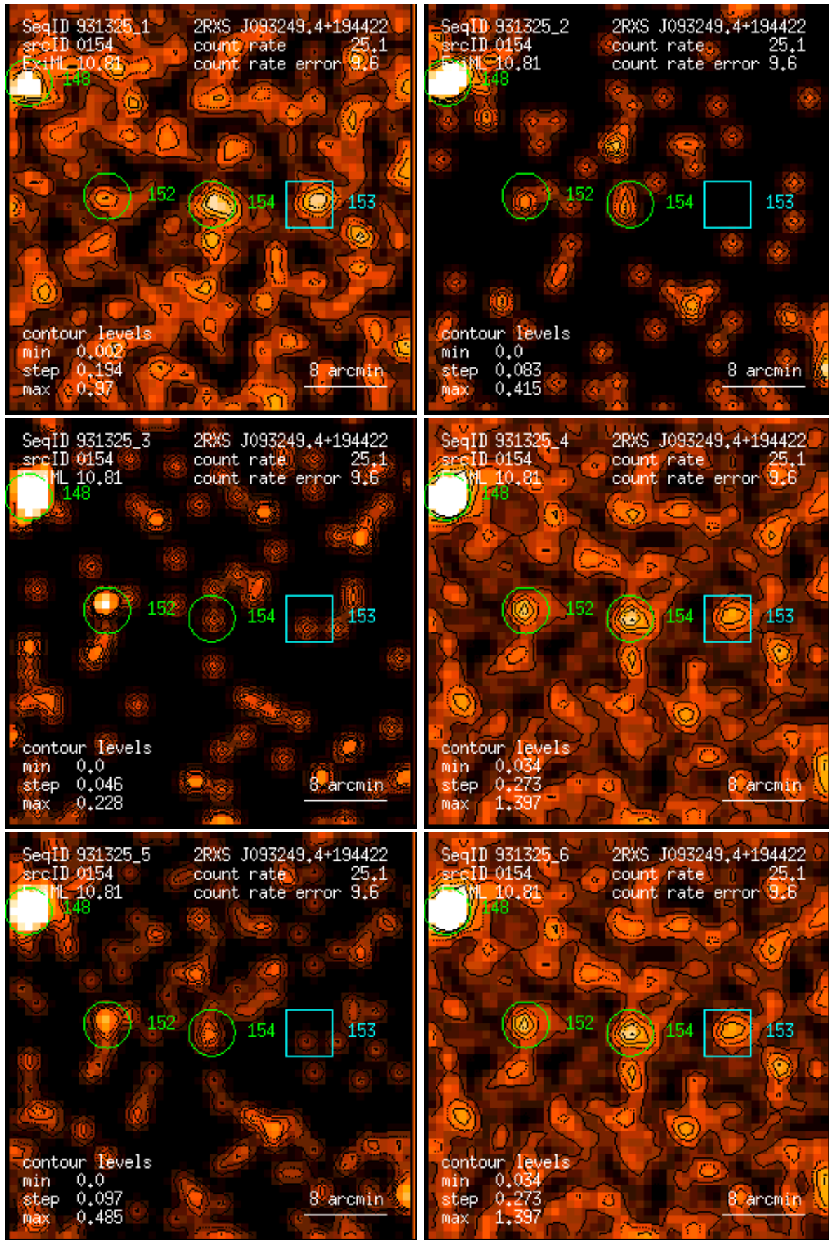
Figure 154: RASS 931325: detection 0154: band rate images, Gaussian filter: (1) PSPC channels 11 – 41, (2) 52 – 90, (3) 91 – 201, (4) 11 – 235, (5) 52 – 201, (6) 11 – 201. Broad band rates in counts/ks. Band rate contour levels in counts/ks/arcmin 2 .
