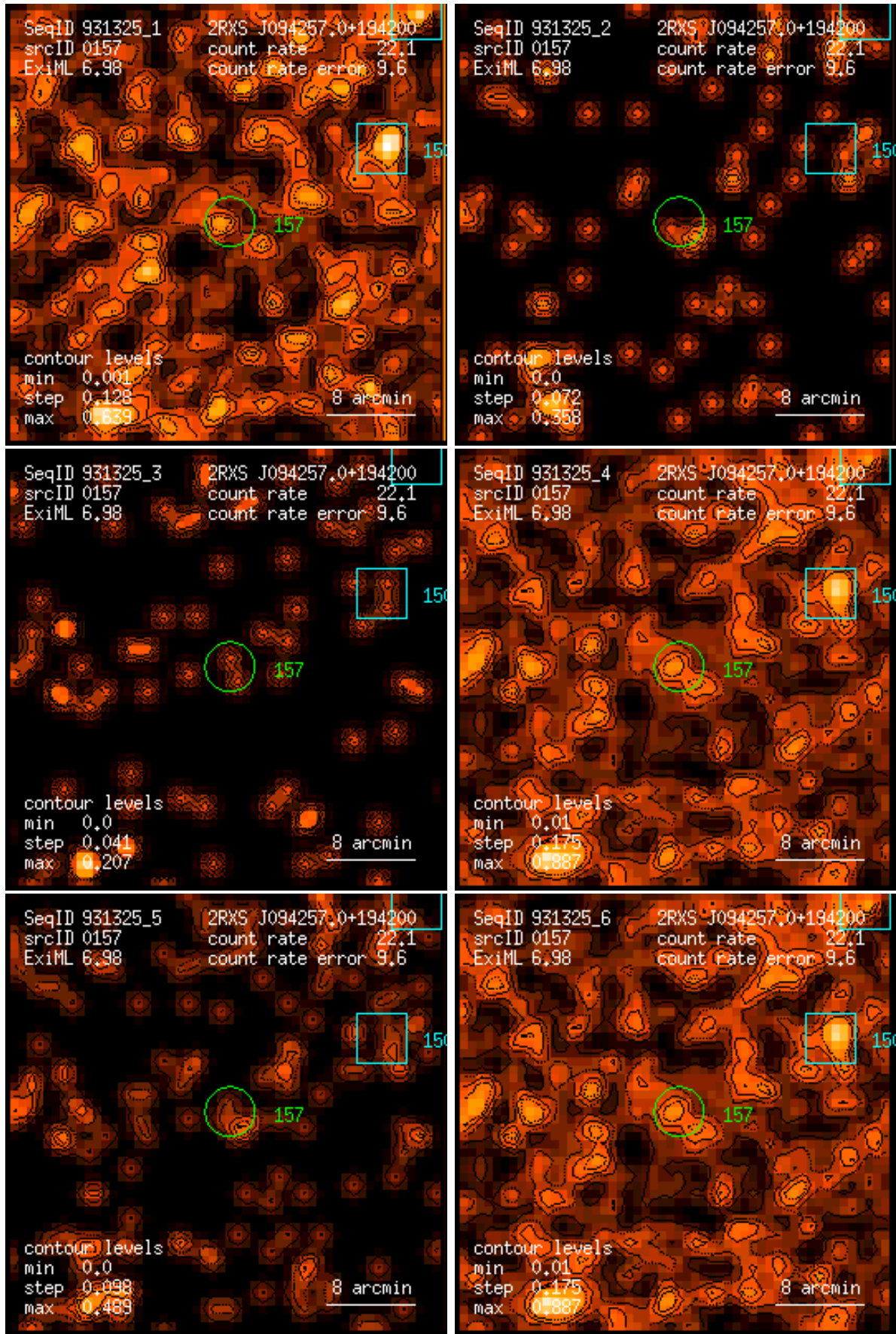
Figure 157: RASS 931325: detection 0157: band rate images, Gaussian filter: (1) PSPC channels 11 – 41, (2) 52 – 90, (3) 91 – 201, (4) 11 – 235, (5) 52 – 201, (6) 11 – 201. Broad band rates in counts/ks. Band rate contour levels in counts/ks/arcmin 2 .
