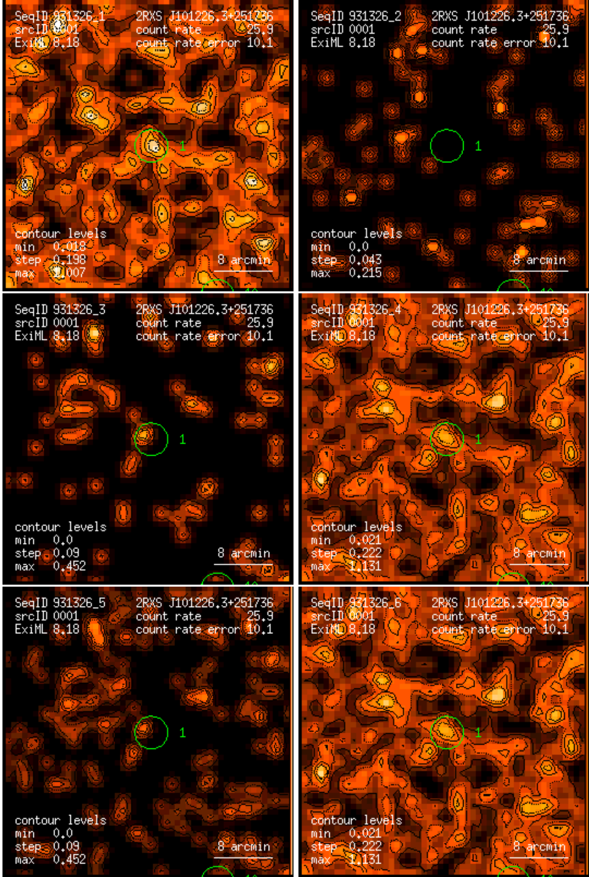
Figure 1: RASS 931326: detection 0001: band rate images, Gaussian filter: (1) PSPC channels 11 – 41, (2) 52 – 90, (3) 91 – 201, (4) 11 – 235, (5) 52 – 201, (6) 11 – 201. Broad band rates in counts/ks. Band rate contour levels in counts/ks/arcmin 2 .
