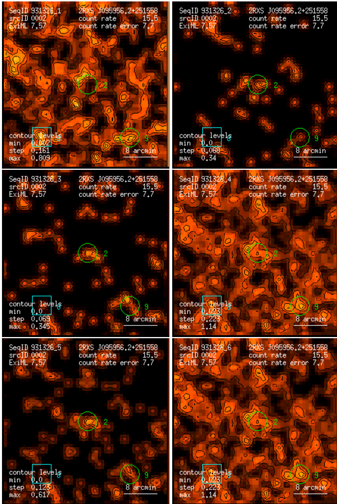
Figure 2: RASS 931326: detection 0002: band rate images, Gaussian filter: (1) PSPC channels 11 – 41, (2) 52 – 90, (3) 91 – 201, (4) 11 – 235, (5) 52 – 201, (6) 11 – 201. Broad band rates in counts/ks. Band rate contour levels in counts/ks/arcmin 2 .
