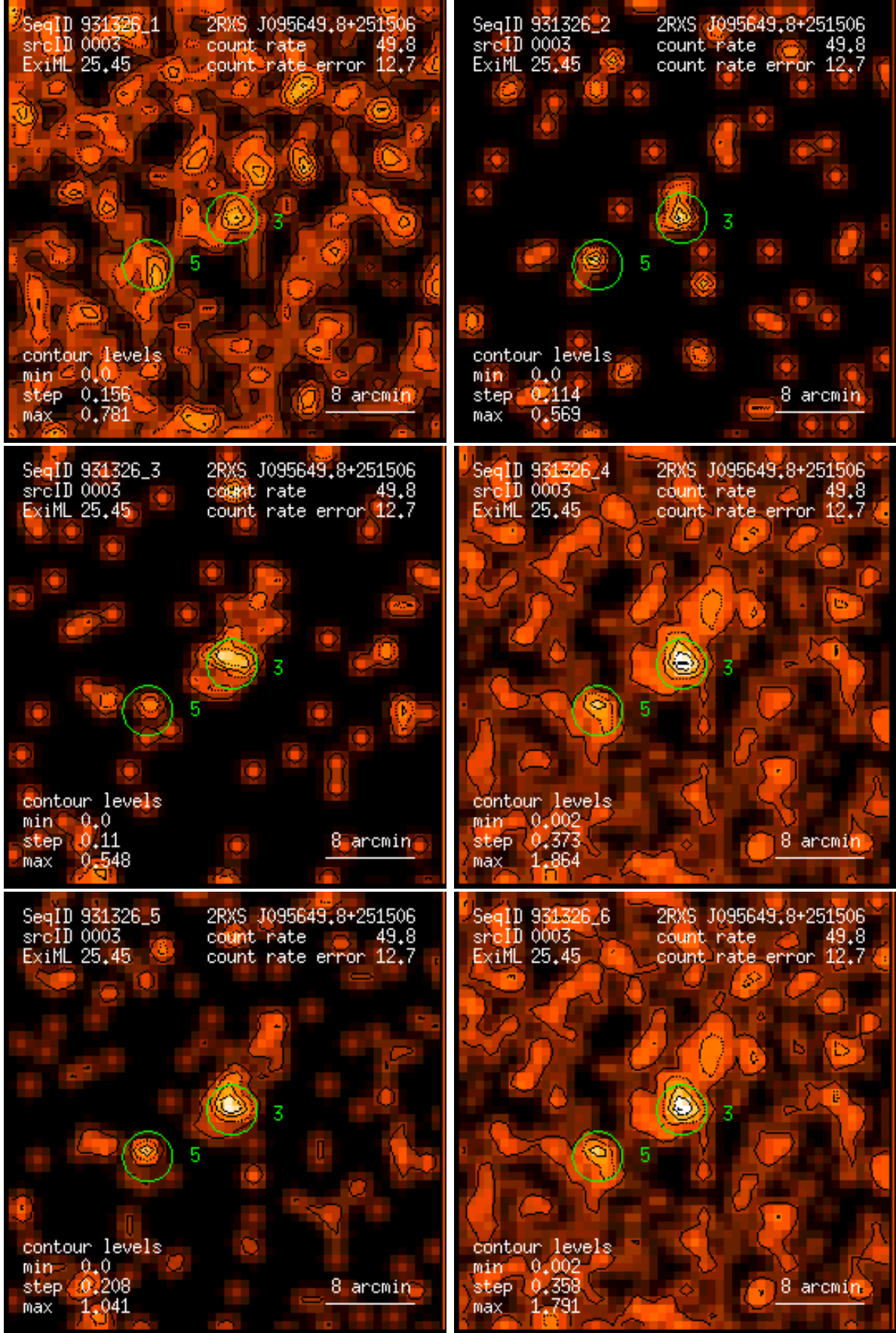
Figure 3: RASS 931326: detection 0003: band rate images, Gaussian filter: (1) PSPC channels 11 – 41, (2) 52 – 90, (3) 91 – 201, (4) 11 – 235, (5) 52 – 201, (6) 11 – 201. Broad band rates in counts/ks. Band rate contour levels in counts/ks/arcmin 2 .
