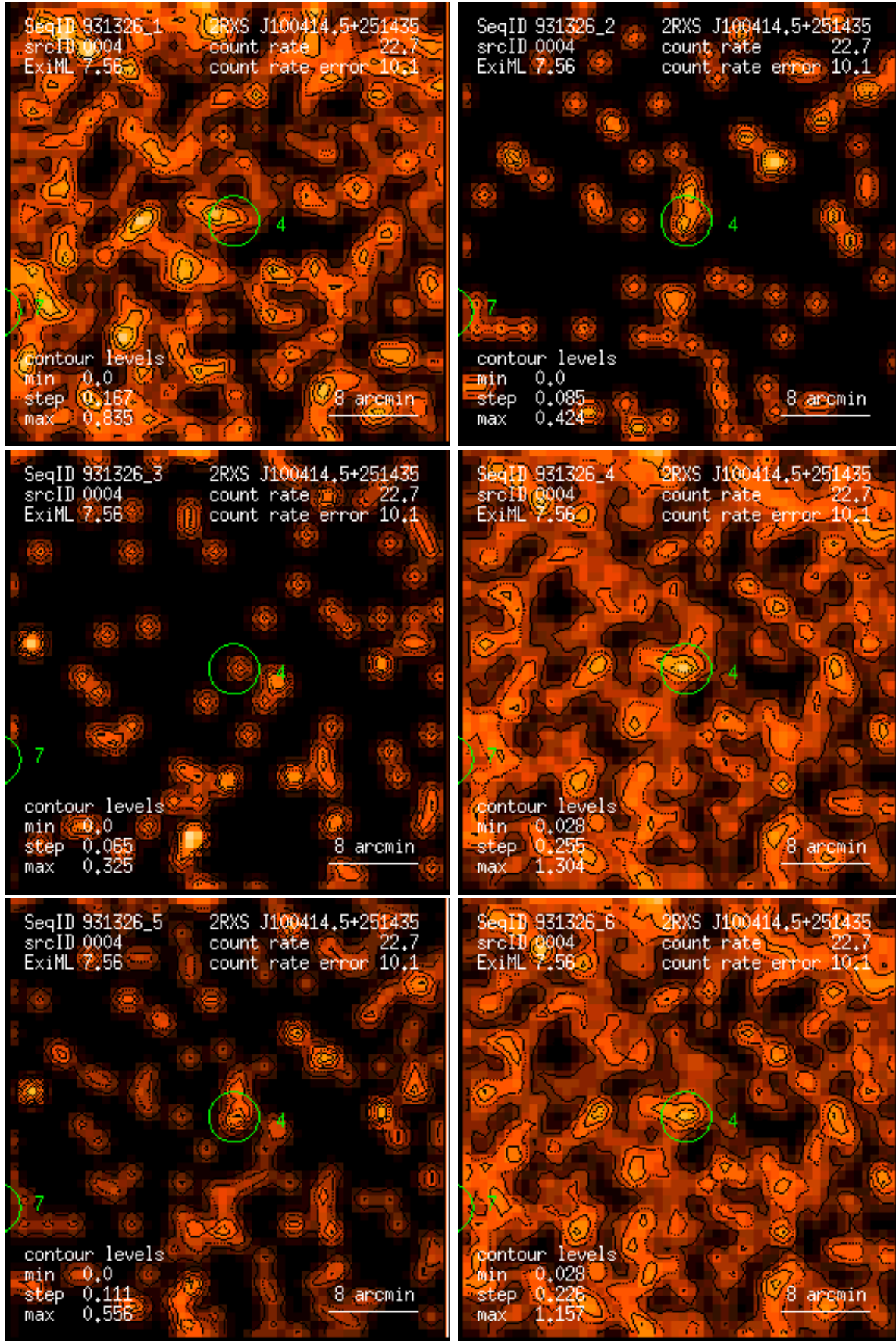
Figure 4: RASS 931326: detection 0004: band rate images, Gaussian filter: (1) PSPC channels 11 – 41, (2) 52 – 90, (3) 91 – 201, (4) 11 – 235, (5) 52 – 201, (6) 11 – 201. Broad band rates in counts/ks. Band rate contour levels in counts/ks/arcmin 2 .
