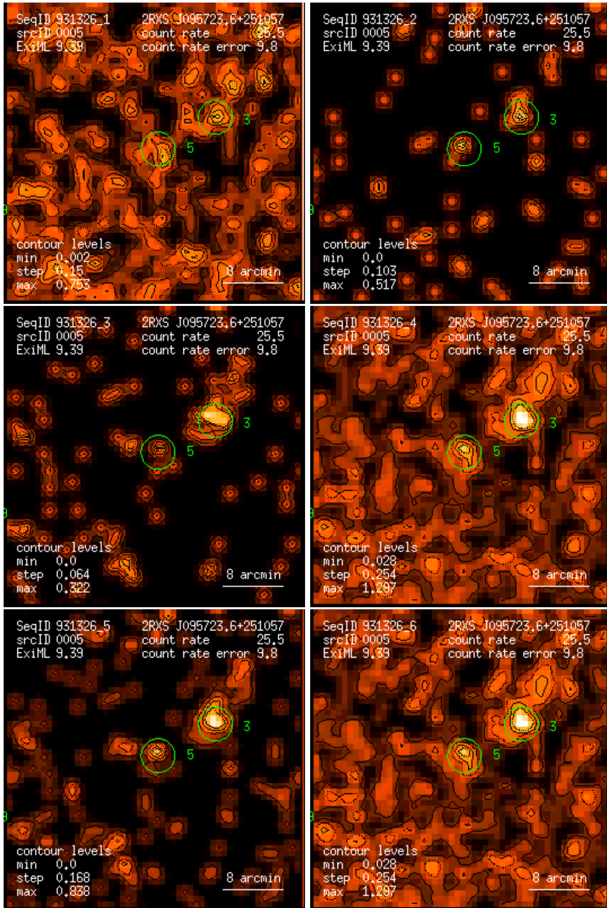
Figure 5: RASS 931326: detection 0005: band rate images, Gaussian filter: (1) PSPC channels 11 – 41, (2) 52 – 90, (3) 91 – 201, (4) 11 – 235, (5) 52 – 201, (6) 11 – 201. Broad band rates in counts/ks. Band rate contour levels in counts/ks/arcmin 2 .
