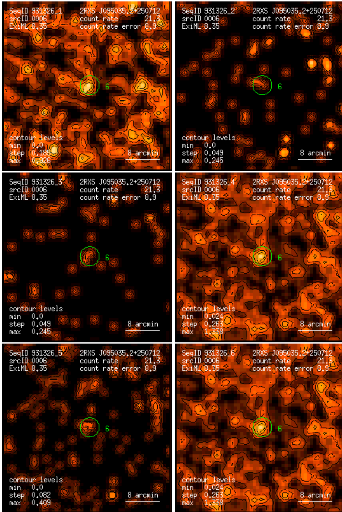
Figure 6: RASS 931326: detection 0006: band rate images, Gaussian filter: (1) PSPC channels 11 – 41, (2) 52 – 90, (3) 91 – 201, (4) 11 – 235, (5) 52 – 201, (6) 11 – 201. Broad band rates in counts/ks. Band rate contour levels in counts/ks/arcmin 2 .
