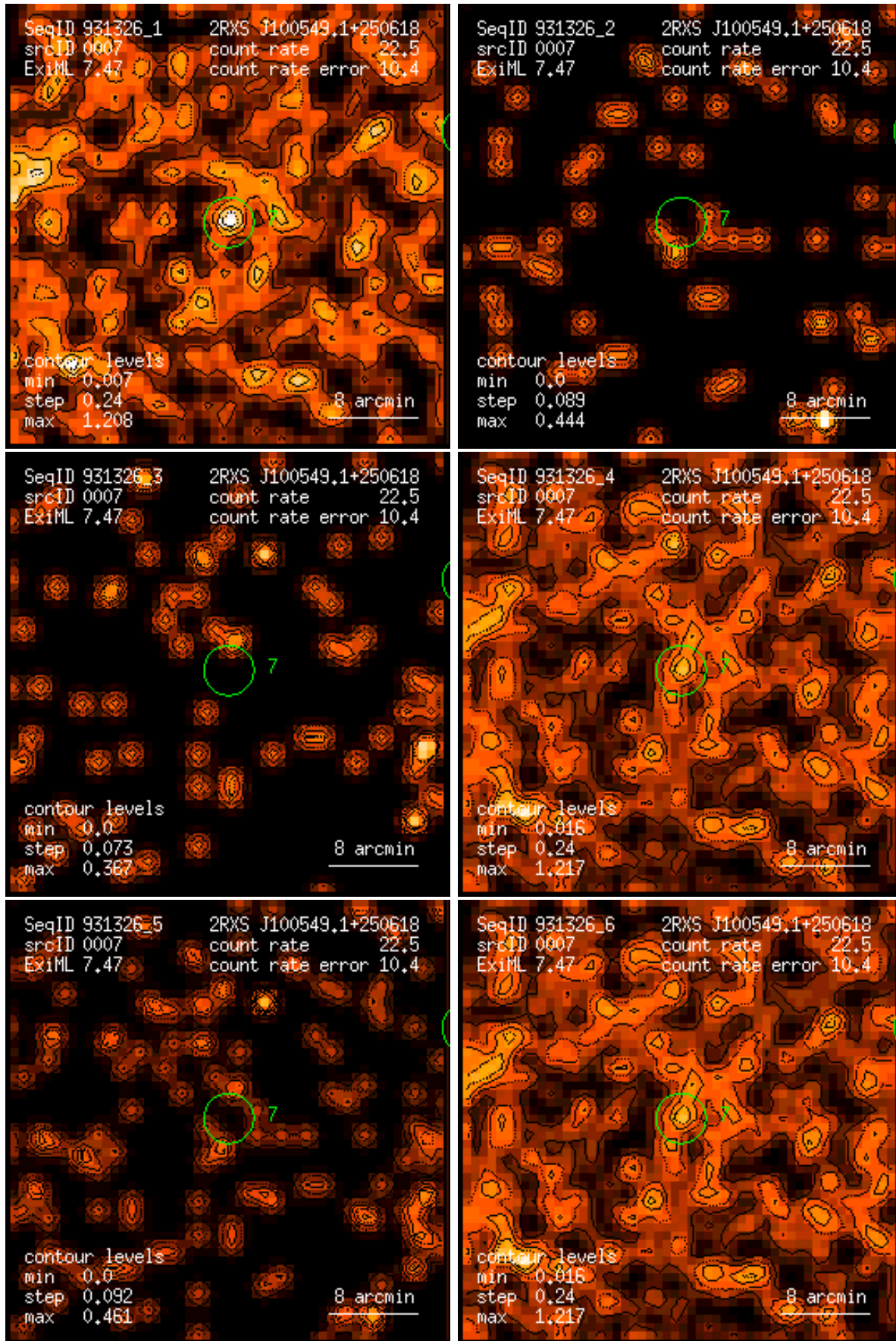
Figure 7: RASS 931326: detection 0007: band rate images, Gaussian filter: (1) PSPC channels 11 – 41, (2) 52 – 90, (3) 91 – 201, (4) 11 – 235, (5) 52 – 201, (6) 11 – 201. Broad band rates in counts/ks. Band rate contour levels in counts/ks/arcmin 2 .
