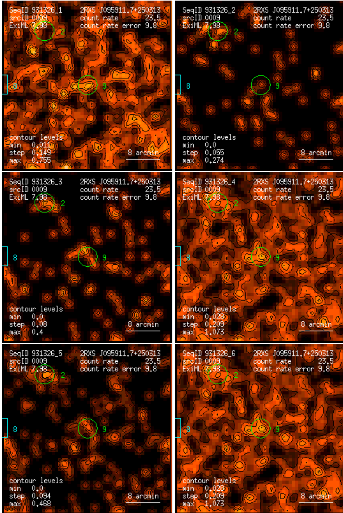
Figure 9: RASS 931326: detection 0009: band rate images, Gaussian filter: (1) PSPC channels 11 – 41, (2) 52 – 90, (3) 91 – 201, (4) 11 – 235, (5) 52 – 201, (6) 11 – 201. Broad band rates in counts/ks. Band rate contour levels in counts/ks/arcmin 2 .
