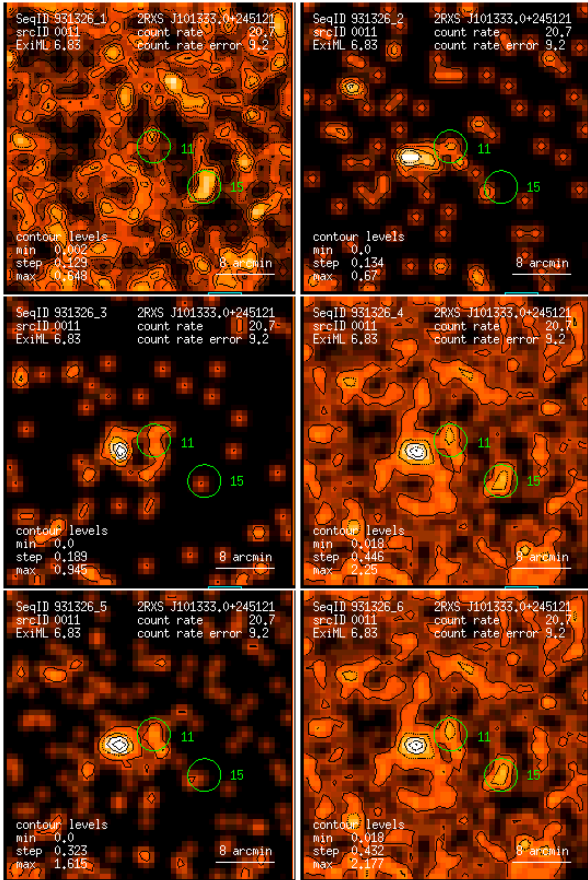
Figure 11: RASS 931326: detection 0011: band rate images, Gaussian filter: (1) PSPC channels 11 – 41, (2) 52 – 90, (3) 91 – 201, (4) 11 – 235, (5) 52 – 201, (6) 11 – 201. Broad band rates in counts/ks. Band rate contour levels in counts/ks/arcmin 2 .
