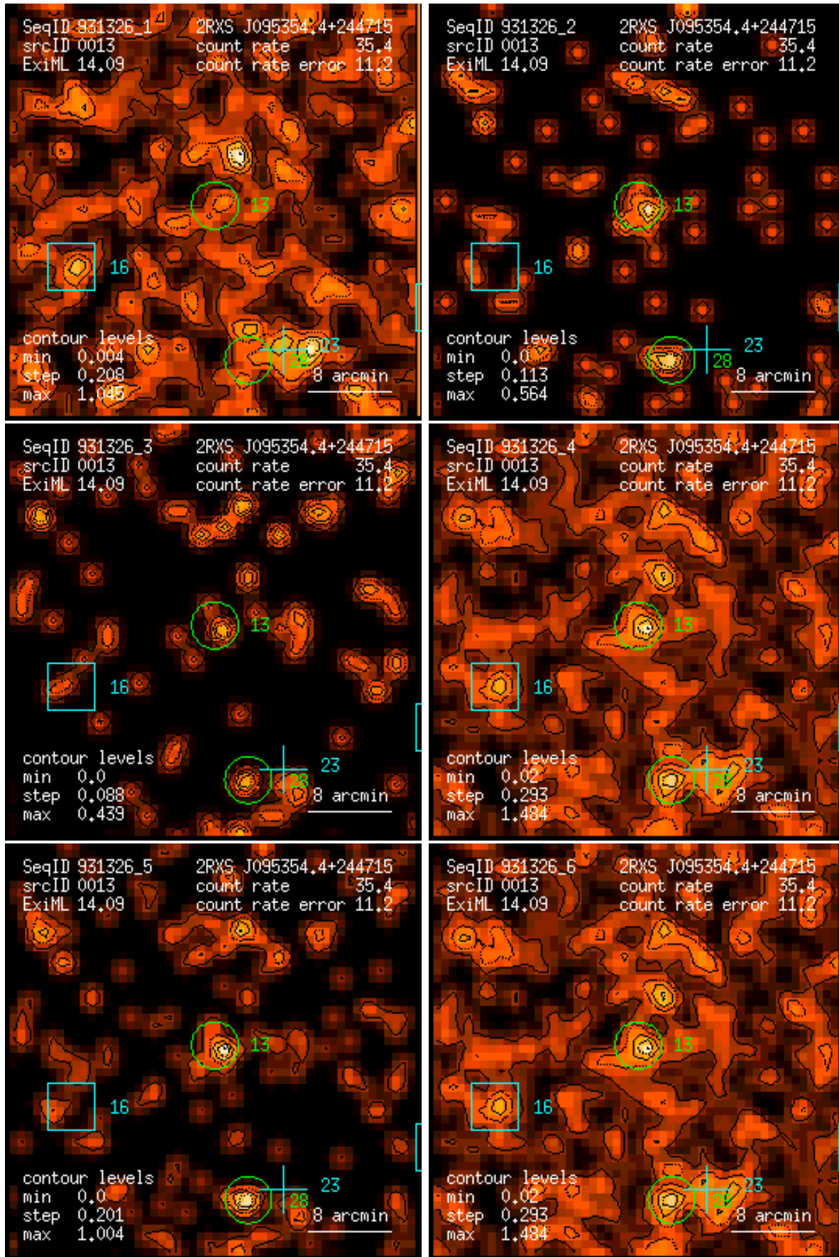
Figure 13: RASS 931326: detection 0013: band rate images, Gaussian filter: (1) PSPC channels 11 – 41, (2) 52 – 90, (3) 91 – 201, (4) 11 – 235, (5) 52 – 201, (6) 11 – 201. Broad band rates in counts/ks. Band rate contour levels in counts/ks/arcmin 2 .
