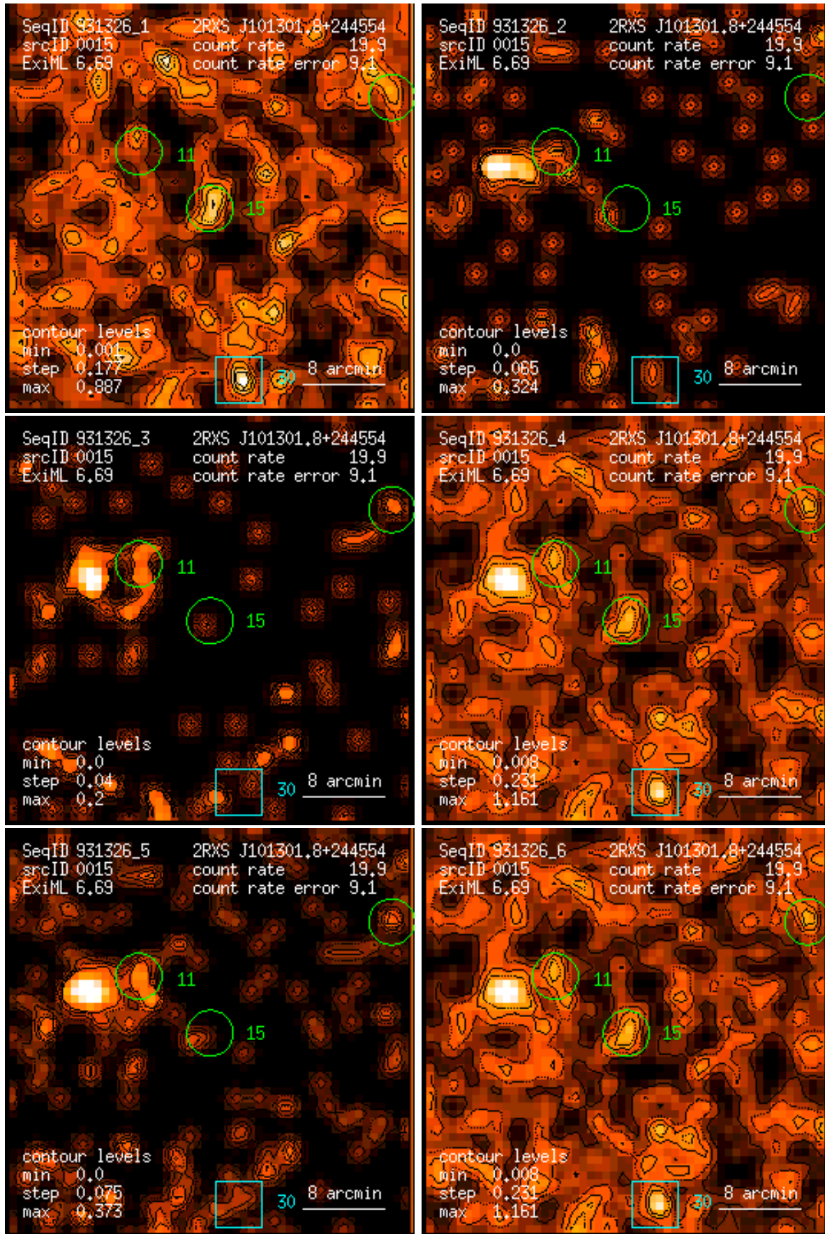
Figure 15: RASS 931326: detection 0015: band rate images, Gaussian filter: (1) PSPC channels 11 – 41, (2) 52 – 90, (3) 91 – 201, (4) 11 – 235, (5) 52 – 201, (6) 11 – 201. Broad band rates in counts/ks. Band rate contour levels in counts/ks/arcmin 2 .
