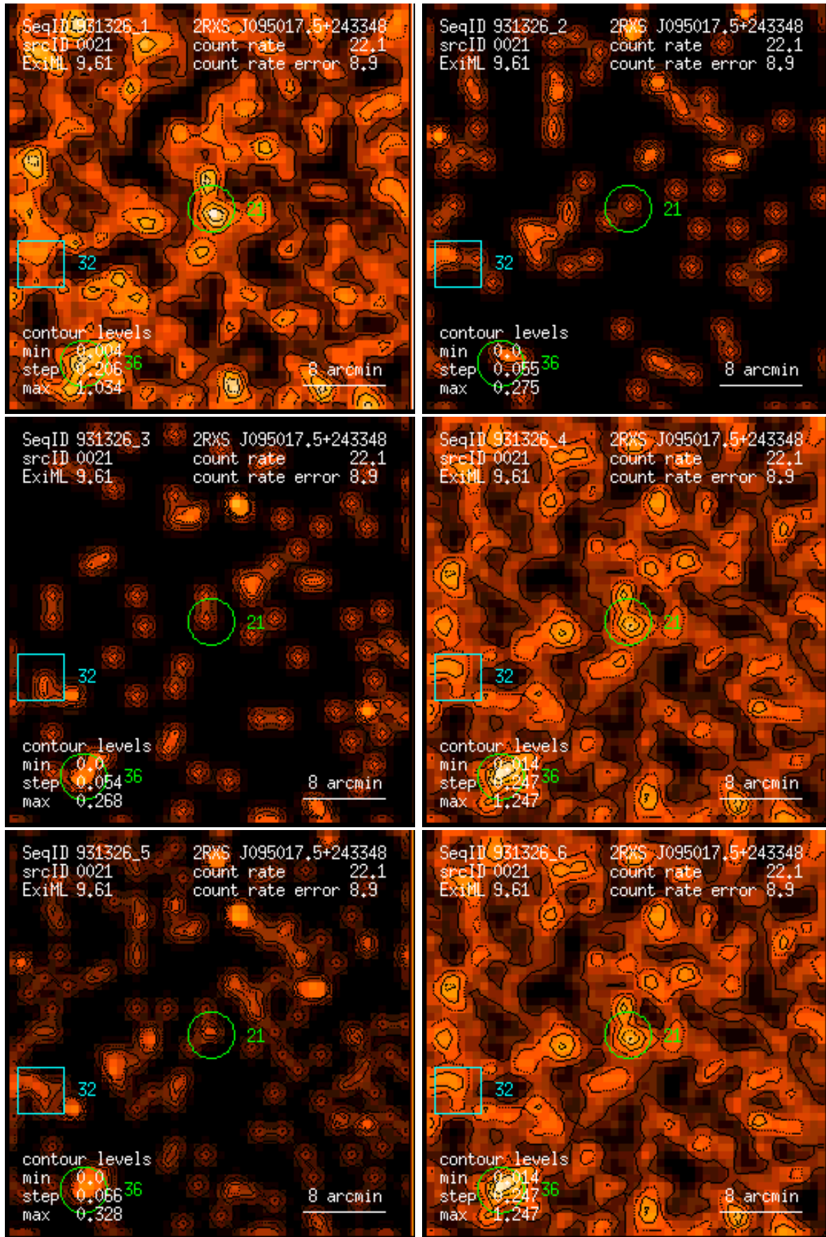
Figure 21: RASS 931326: detection 0021: band rate images, Gaussian filter: (1) PSPC channels 11 – 41, (2) 52 – 90, (3) 91 – 201, (4) 11 – 235, (5) 52 – 201, (6) 11 – 201. Broad band rates in counts/ks. Band rate contour levels in counts/ks/arcmin 2 .
