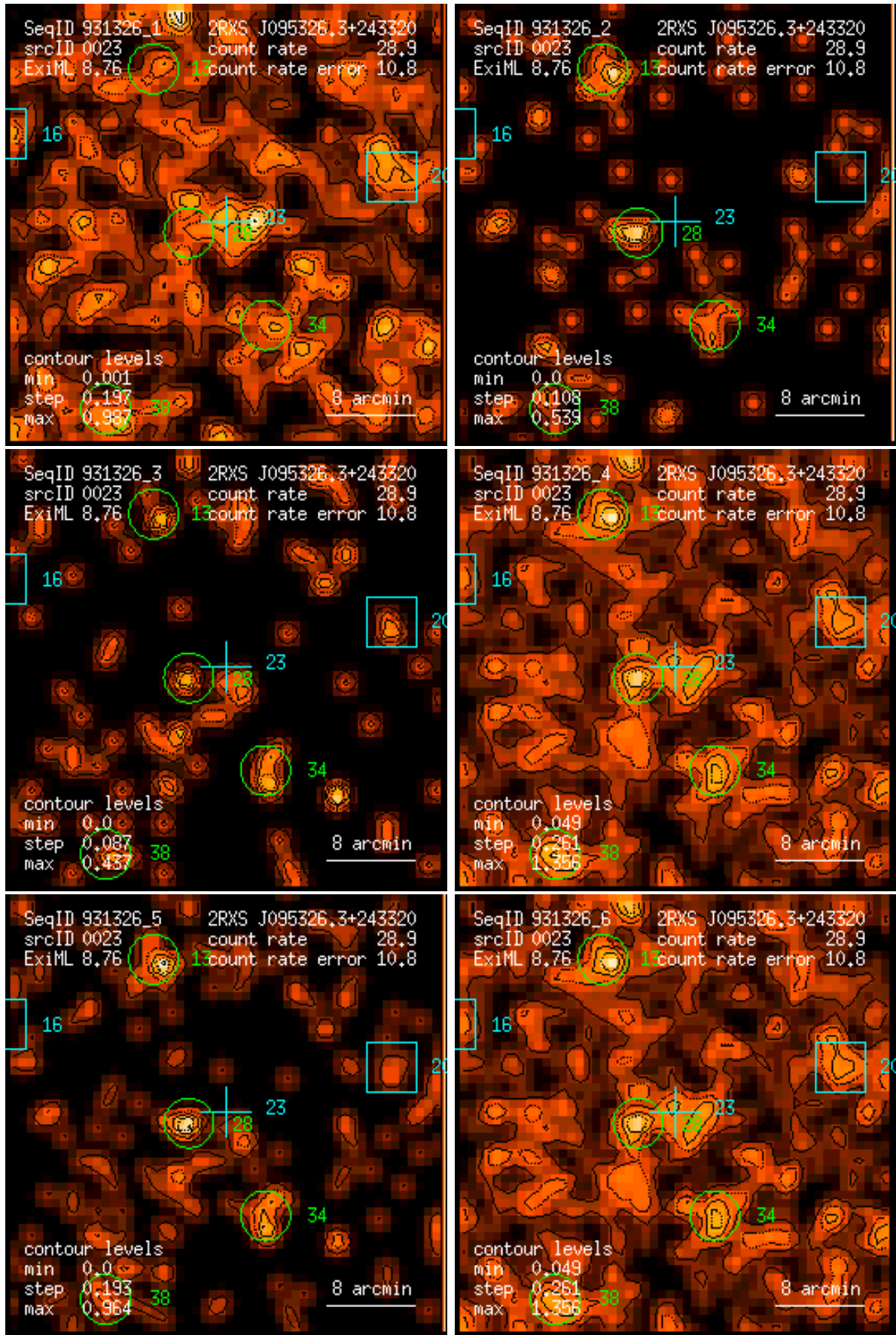
Figure 23: RASS 931326: detection 0023: band rate images, Gaussian filter: (1) PSPC channels 11 – 41, (2) 52 – 90, (3) 91 – 201, (4) 11 – 235, (5) 52 – 201, (6) 11 – 201. Broad band rates in counts/ks. Band rate contour levels in counts/ks/arcmin 2 .
