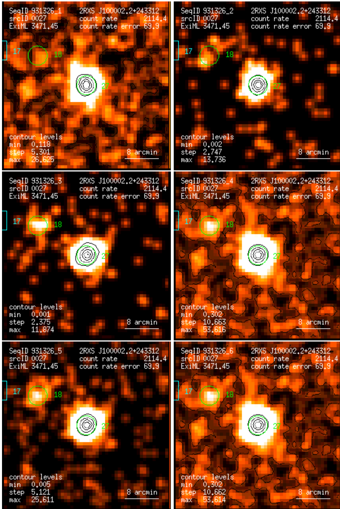
Figure 27: RASS 931326: detection 0027: band rate images, Gaussian filter: (1) PSPC channels 11 – 41, (2) 52 – 90, (3) 91 – 201, (4) 11 – 235, (5) 52 – 201, (6) 11 – 201. Broad band rates in counts/ks. Band rate contour levels in counts/ks/arcmin 2 .
