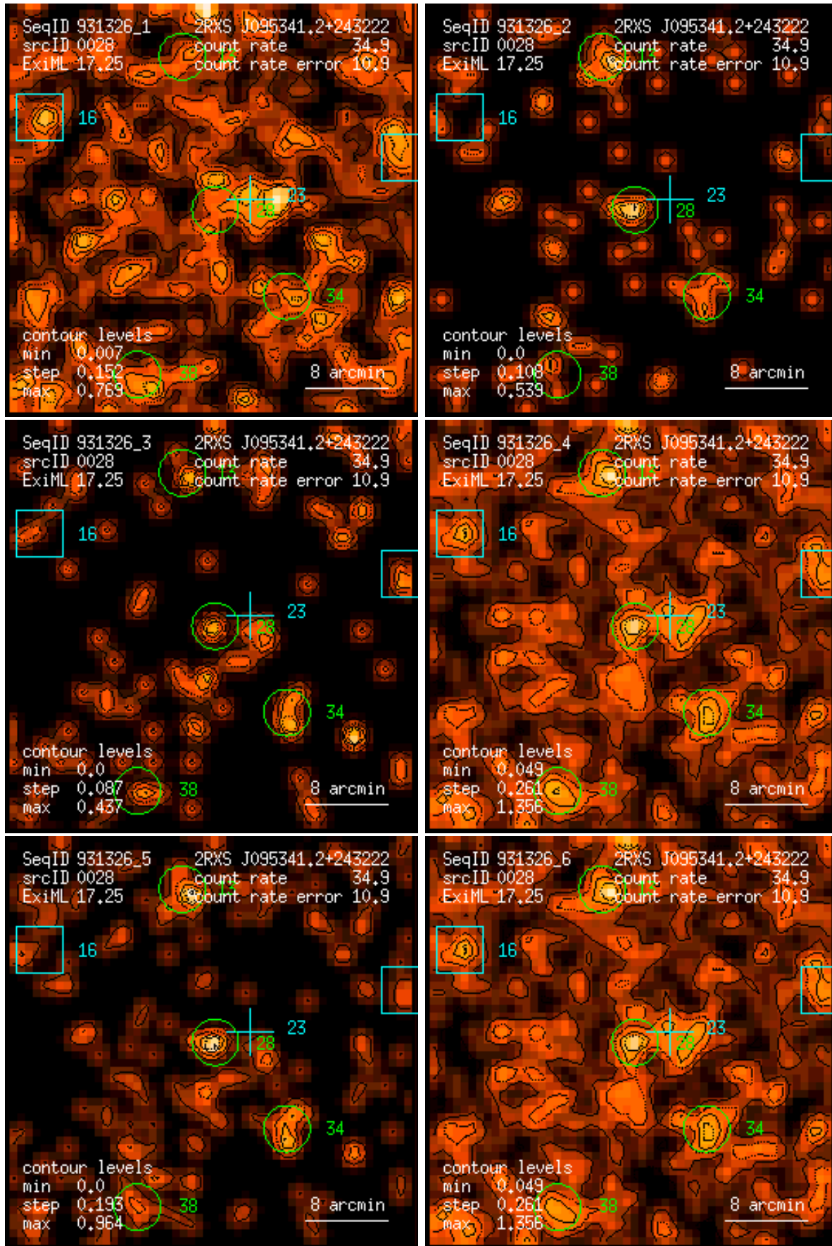
Figure 28: RASS 931326: detection 0028: band rate images, Gaussian filter: (1) PSPC channels 11 – 41, (2) 52 – 90, (3) 91 – 201, (4) 11 – 235, (5) 52 – 201, (6) 11 – 201. Broad band rates in counts/ks. Band rate contour levels in counts/ks/arcmin 2 .
