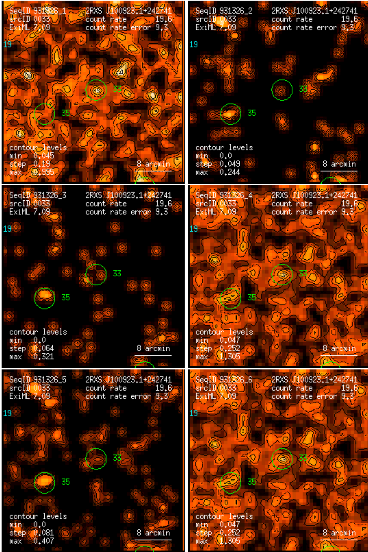
Figure 33: RASS 931326: detection 0033: band rate images, Gaussian filter: (1) PSPC channels 11 – 41, (2) 52 – 90, (3) 91 – 201, (4) 11 – 235, (5) 52 – 201, (6) 11 – 201. Broad band rates in counts/ks. Band rate contour levels in counts/ks/arcmin 2 .
