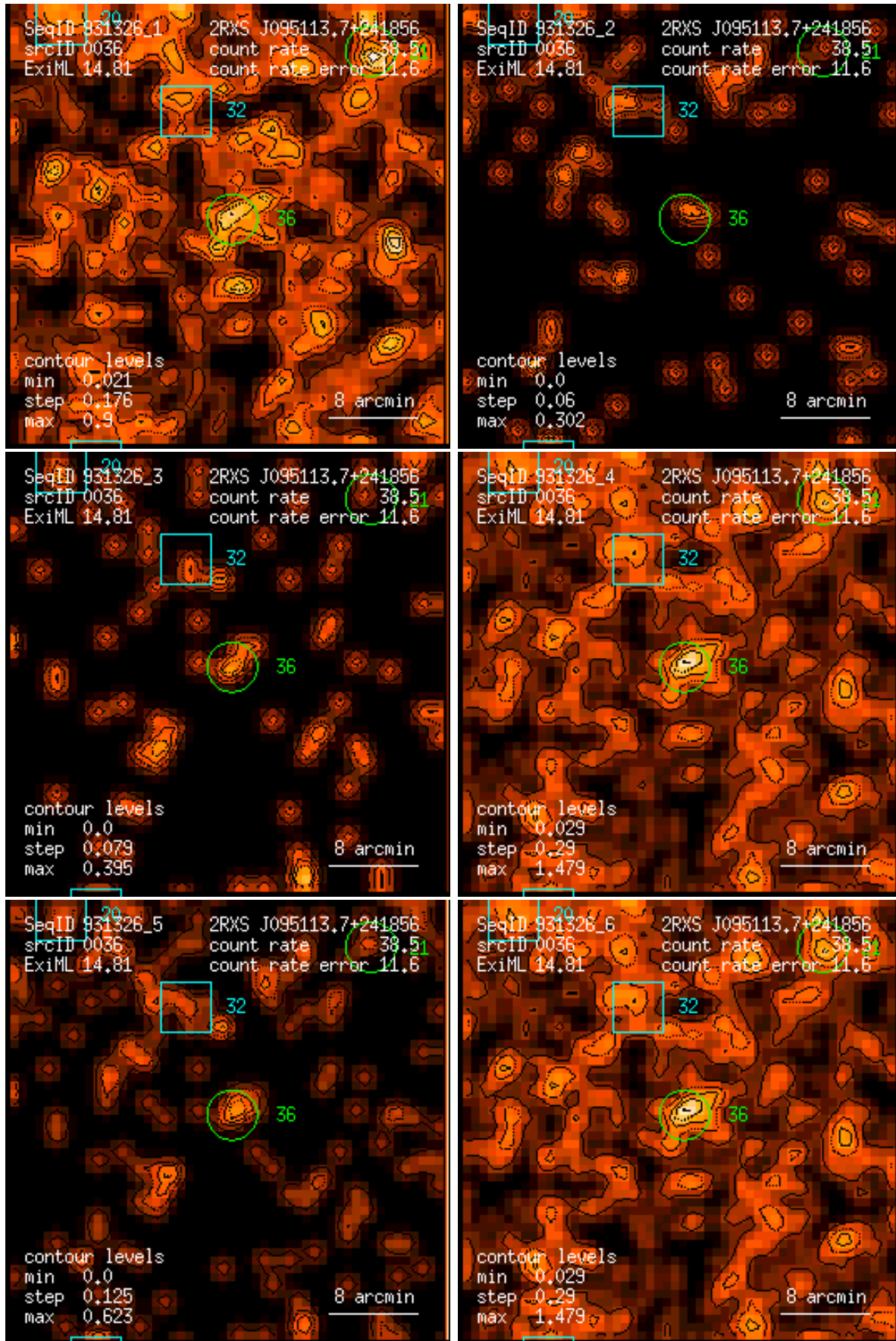
Figure 36: RASS 931326: detection 0036: band rate images, Gaussian filter: (1) PSPC channels 11 – 41, (2) 52 – 90, (3) 91 – 201, (4) 11 – 235, (5) 52 – 201, (6) 11 – 201. Broad band rates in counts/ks. Band rate contour levels in counts/ks/arcmin 2 .
