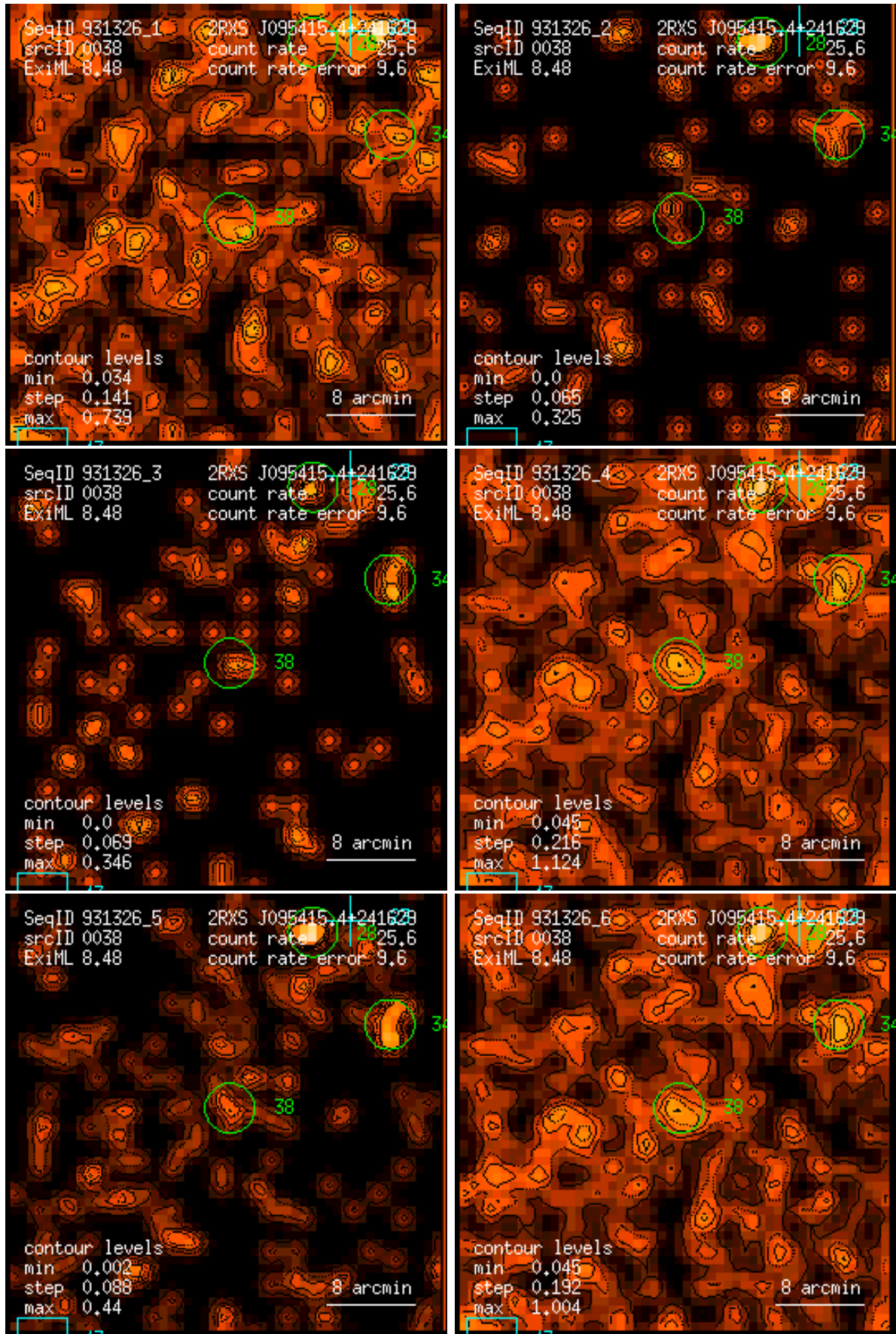
Figure 38: RASS 931326: detection 0038: band rate images, Gaussian filter: (1) PSPC channels 11 – 41, (2) 52 – 90, (3) 91 – 201, (4) 11 – 235, (5) 52 – 201, (6) 11 – 201. Broad band rates in counts/ks. Band rate contour levels in counts/ks/arcmin 2 .
