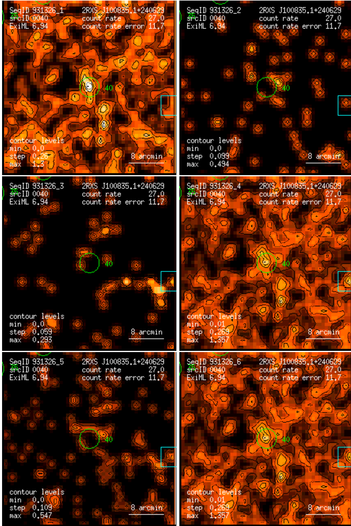
Figure 40: RASS 931326: detection 0040: band rate images, Gaussian filter: (1) PSPC channels 11 – 41, (2) 52 – 90, (3) 91 – 201, (4) 11 – 235, (5) 52 – 201, (6) 11 – 201. Broad band rates in counts/ks. Band rate contour levels in counts/ks/arcmin 2 .
