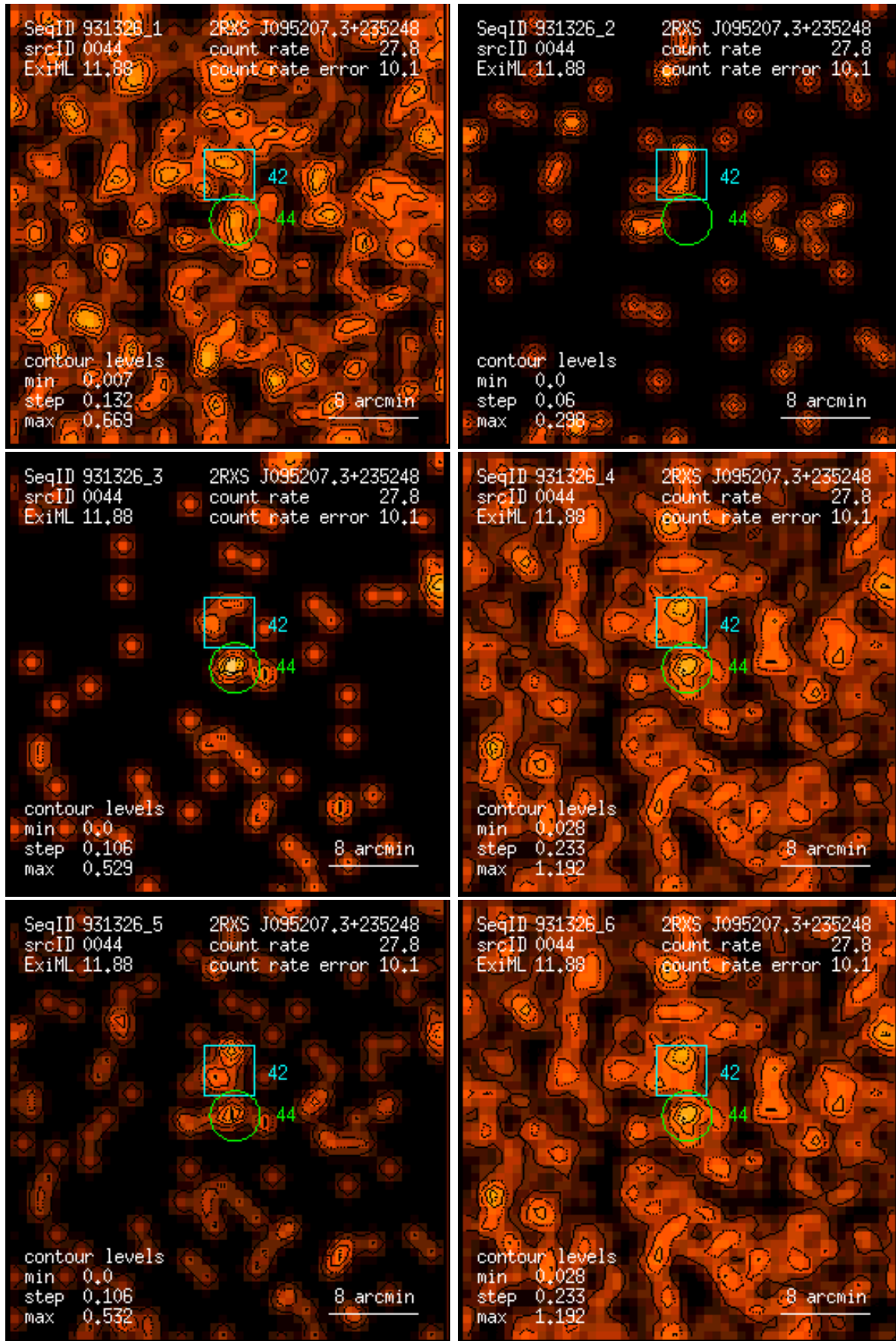
Figure 44: RASS 931326: detection 0044: band rate images, Gaussian filter: (1) PSPC channels 11 – 41, (2) 52 – 90, (3) 91 – 201, (4) 11 – 235, (5) 52 – 201, (6) 11 – 201. Broad band rates in counts/ks. Band rate contour levels in counts/ks/arcmin 2 .
