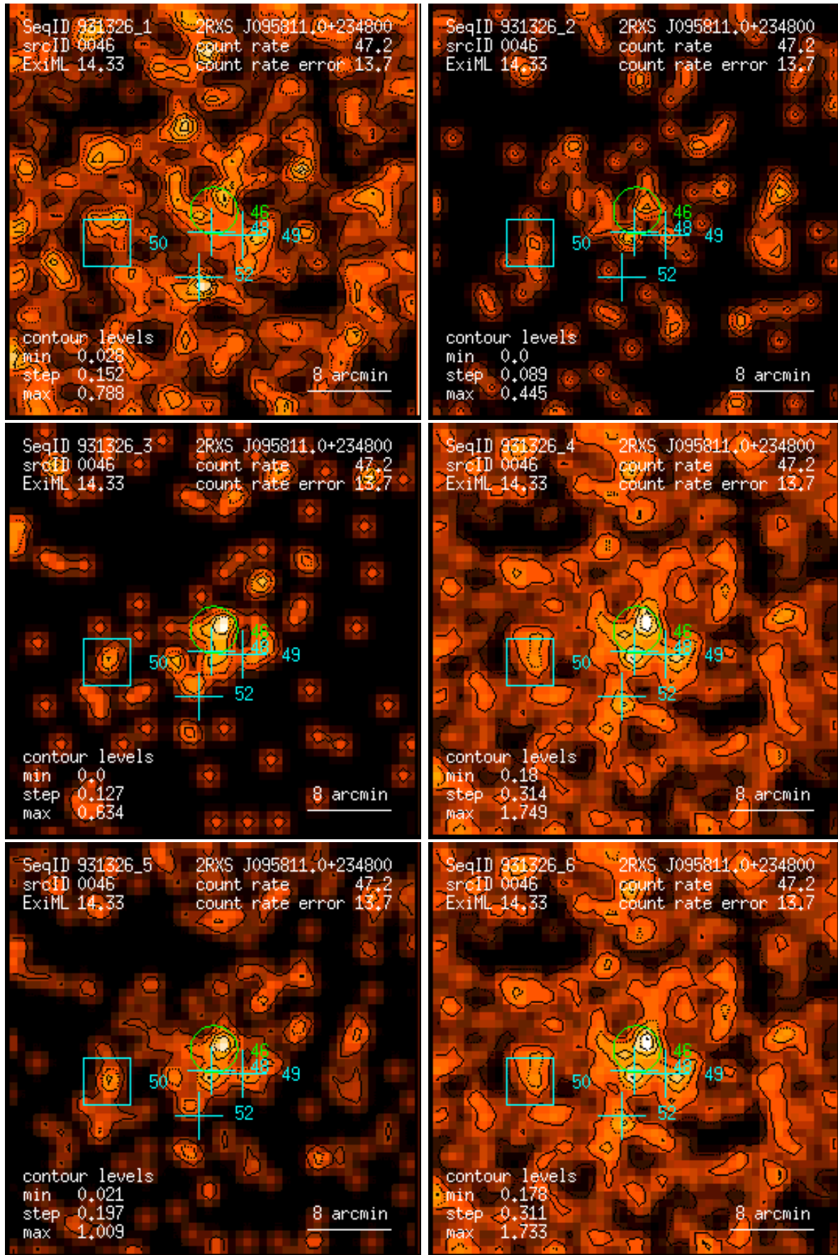
Figure 46: RASS 931326: detection 0046: band rate images, Gaussian filter: (1) PSPC channels 11 – 41, (2) 52 – 90, (3) 91 – 201, (4) 11 – 235, (5) 52 – 201, (6) 11 – 201. Broad band rates in counts/ks. Band rate contour levels in counts/ks/arcmin 2 .
