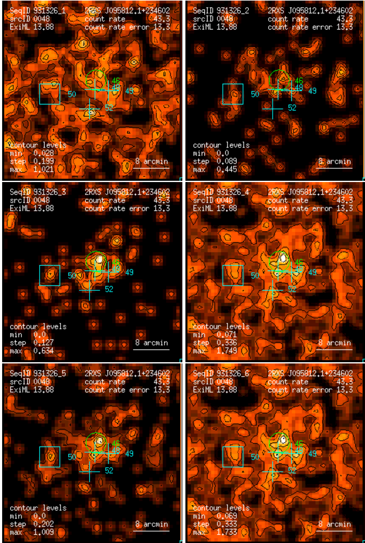
Figure 48: RASS 931326: detection 0048: band rate images, Gaussian filter: (1) PSPC channels 11 – 41, (2) 52 – 90, (3) 91 – 201, (4) 11 – 235, (5) 52 – 201, (6) 11 – 201. Broad band rates in counts/ks. Band rate contour levels in counts/ks/arcmin 2 .
