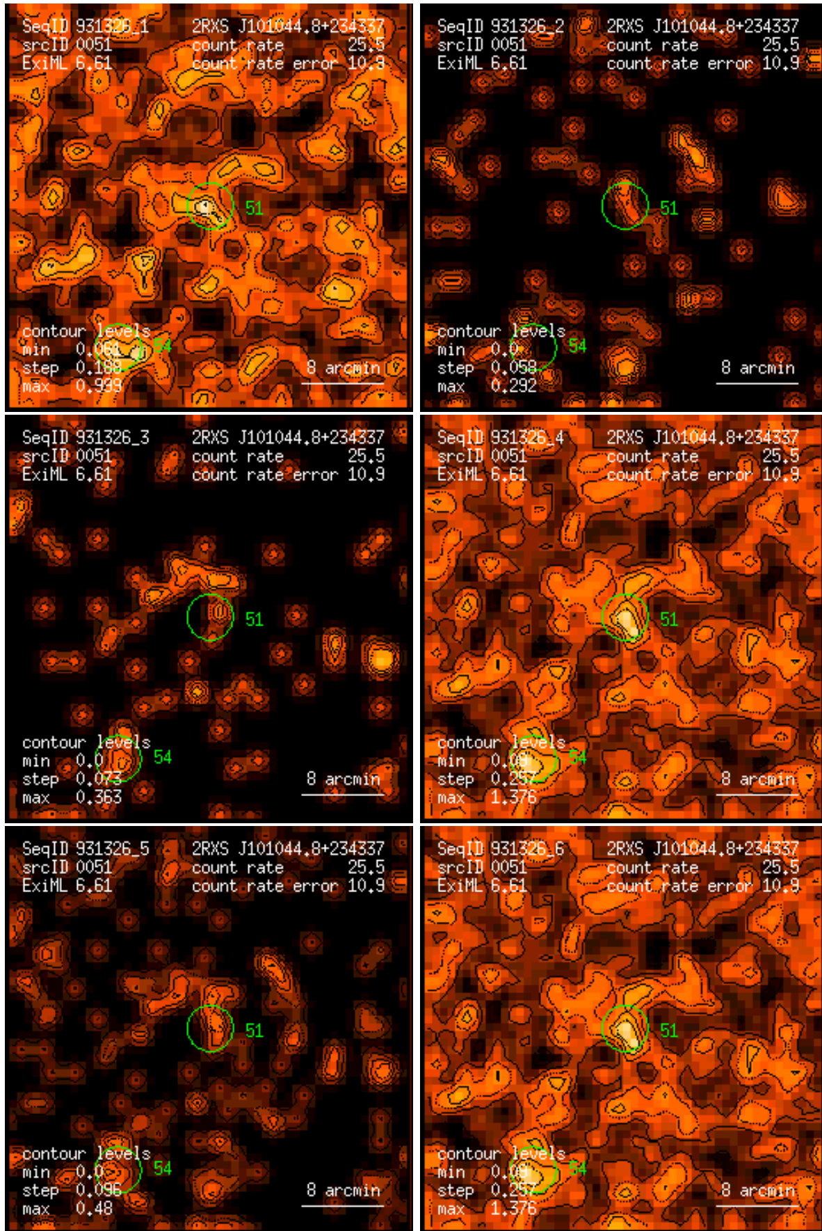
Figure 51: RASS 931326: detection 0051: band rate images, Gaussian filter: (1) PSPC channels 11 – 41, (2) 52 – 90, (3) 91 – 201, (4) 11 – 235, (5) 52 – 201, (6) 11 – 201. Broad band rates in counts/ks. Band rate contour levels in counts/ks/arcmin 2 .
