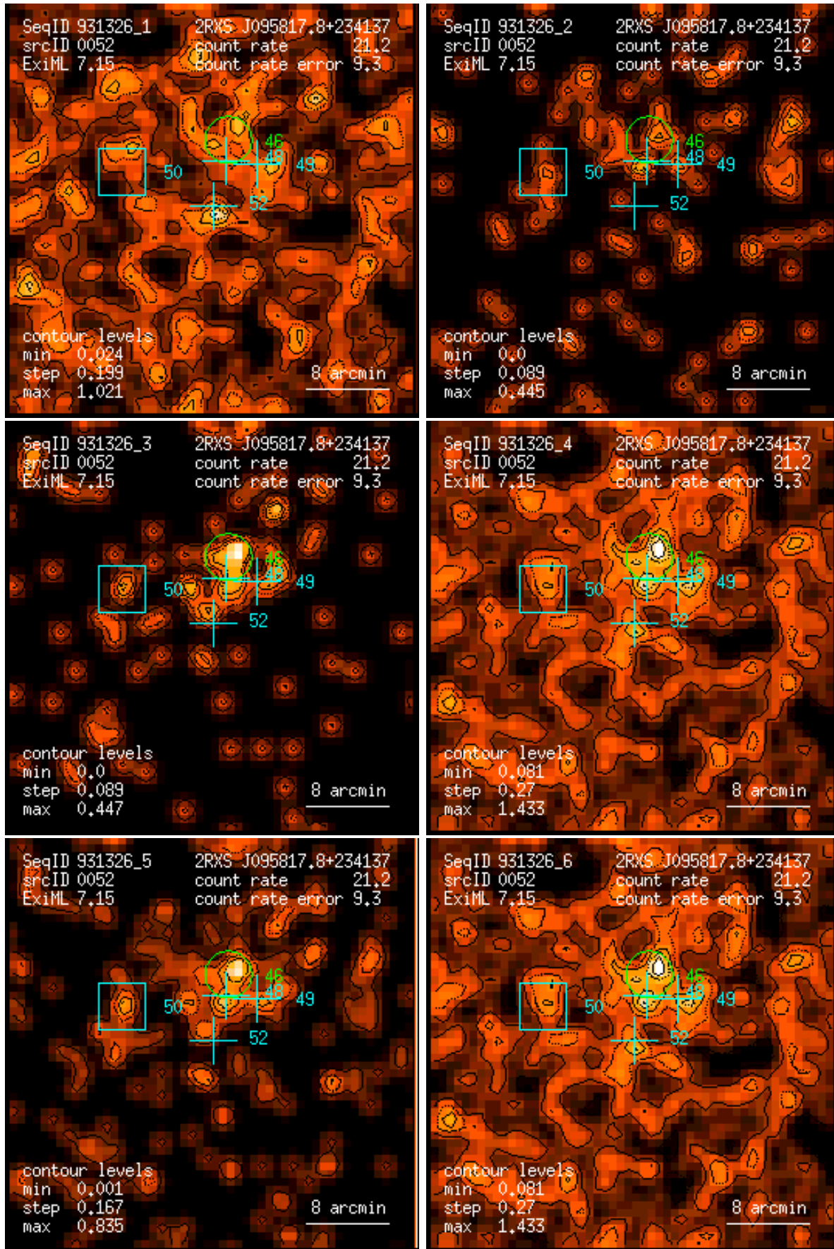
Figure 52: RASS 931326: detection 0052: band rate images, Gaussian filter: (1) PSPC channels 11 – 41, (2) 52 – 90, (3) 91 – 201, (4) 11 – 235, (5) 52 – 201, (6) 11 – 201. Broad band rates in counts/ks. Band rate contour levels in counts/ks/arcmin 2 .
