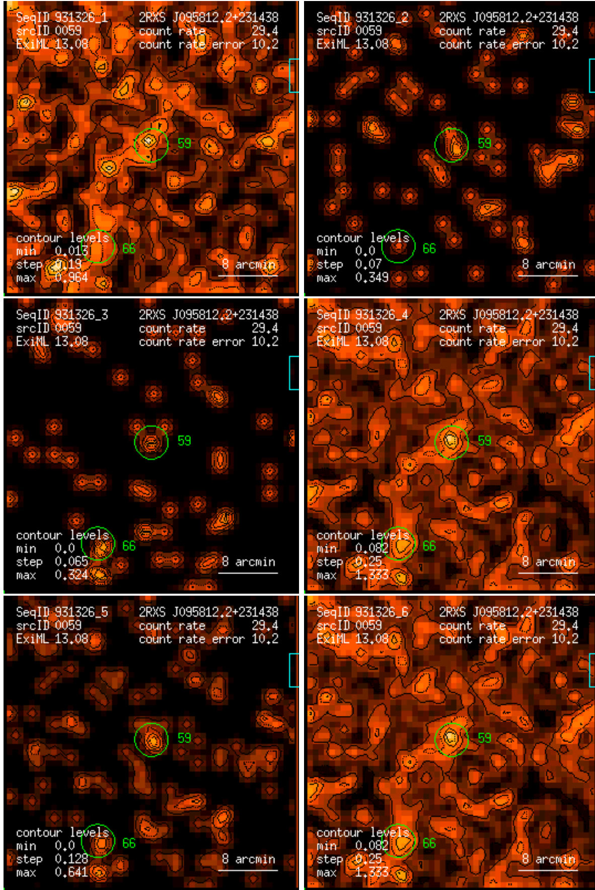
Figure 59: RASS 931326: detection 0059: band rate images, Gaussian filter: (1) PSPC channels 11 – 41, (2) 52 – 90, (3) 91 – 201, (4) 11 – 235, (5) 52 – 201, (6) 11 – 201. Broad band rates in counts/ks. Band rate contour levels in counts/ks/arcmin 2 .
