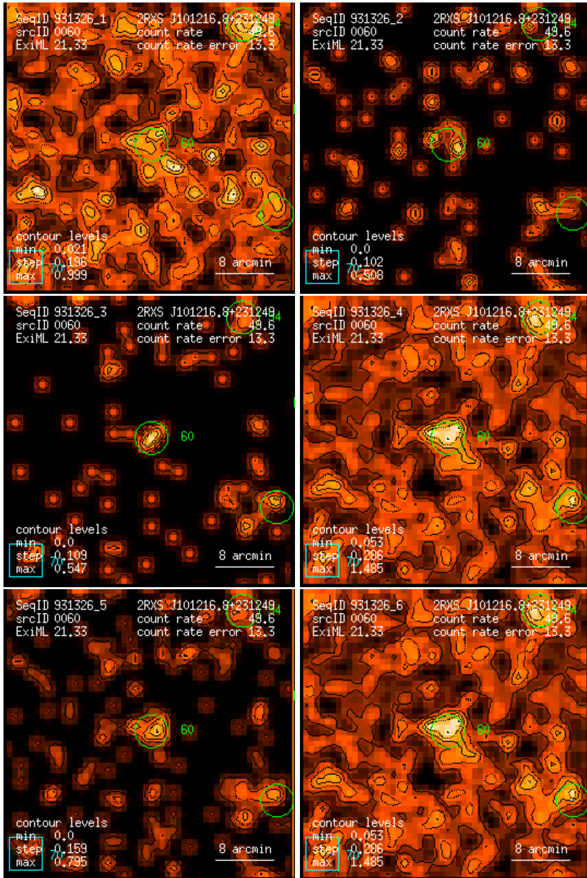
Figure 60: RASS 931326: detection 0060: band rate images, Gaussian filter: (1) PSPC channels 11 – 41, (2) 52 – 90, (3) 91 – 201, (4) 11 – 235, (5) 52 – 201, (6) 11 – 201. Broad band rates in counts/ks. Band rate contour levels in counts/ks/arcmin 2 .
