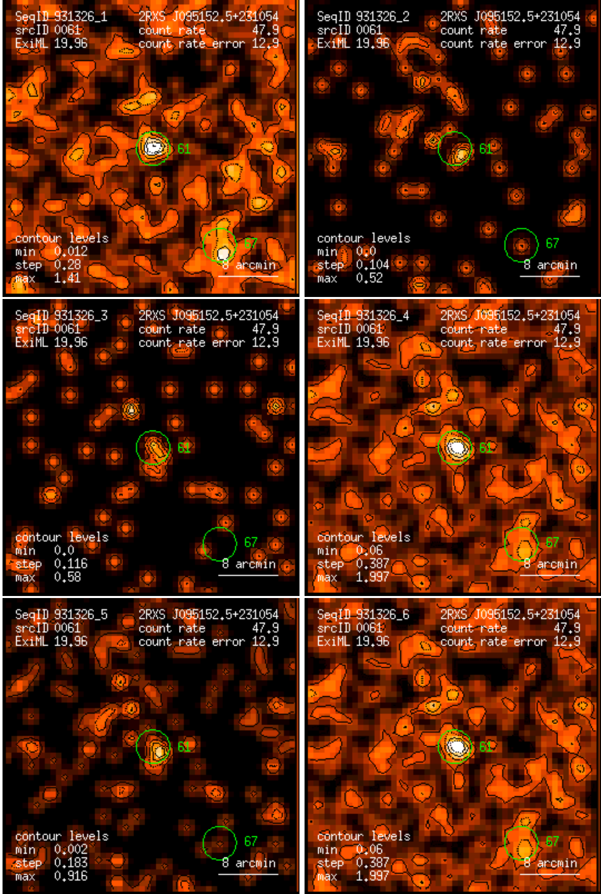
Figure 61: RASS 931326: detection 0061: band rate images, Gaussian filter: (1) PSPC channels 11 – 41, (2) 52 – 90, (3) 91 – 201, (4) 11 – 235, (5) 52 – 201, (6) 11 – 201. Broad band rates in counts/ks. Band rate contour levels in counts/ks/arcmin 2 .
